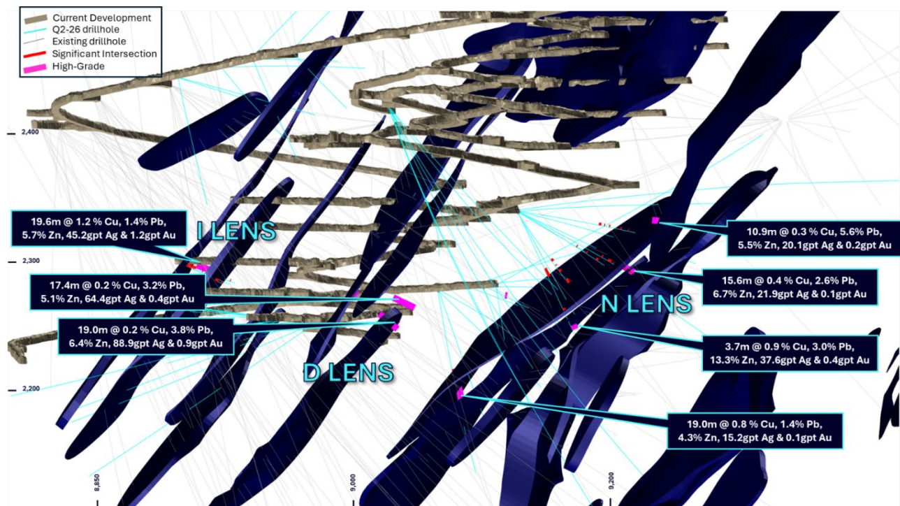
Figure 6 - Woodlawn drilling Dec-25 significant intercepts (North viewing cross section +/-750m)
