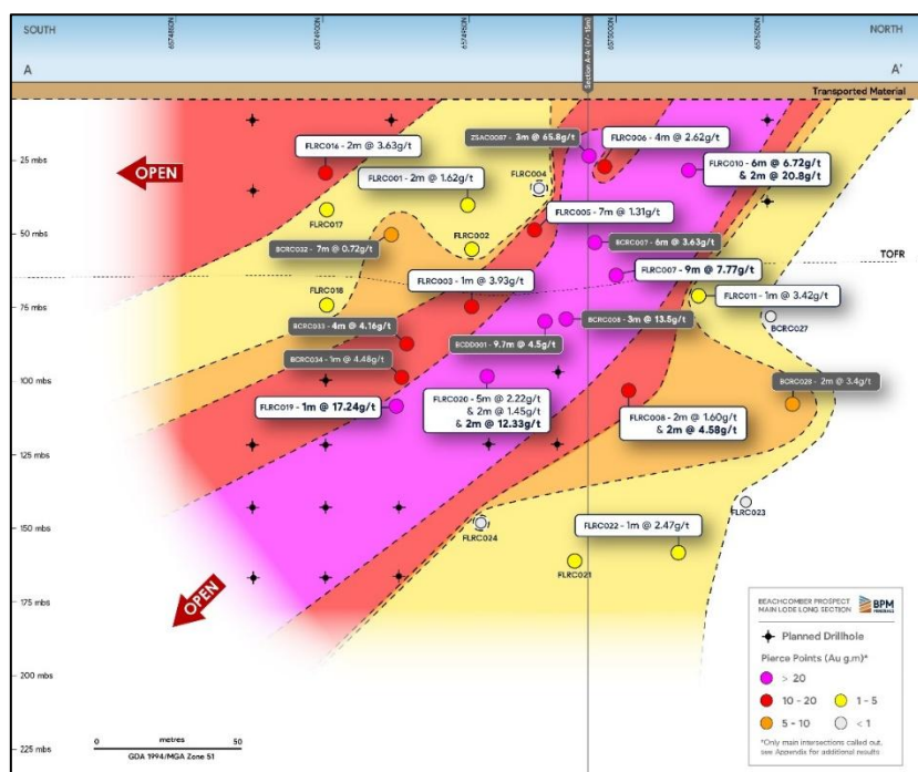
Figure 1 - Beachcomber Long Section (looking west) with a newly-defined high-grade, south-plunging shoot that remains open at depth, to be targeted in upcoming drilling
