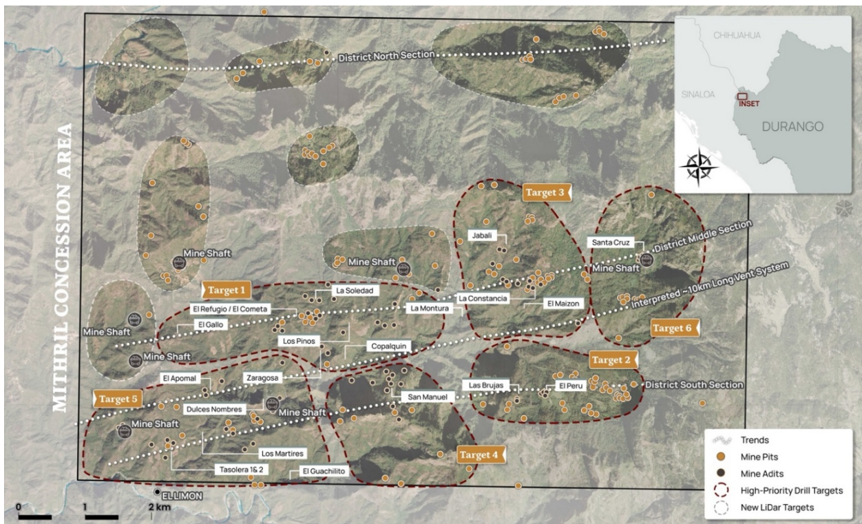
Figure 2 LiDAR identified historic workings across the 70km 2 district. Current drilling locations at Target 1 west and Target 5 (El Apomel), and recent drilling at Zaragosa mine in Target 1 south, high priority drill target area of La Constancia-El Jabali (Target 3). Several new areas highlighted across the district for follow-up work including recently sampled Target 6
