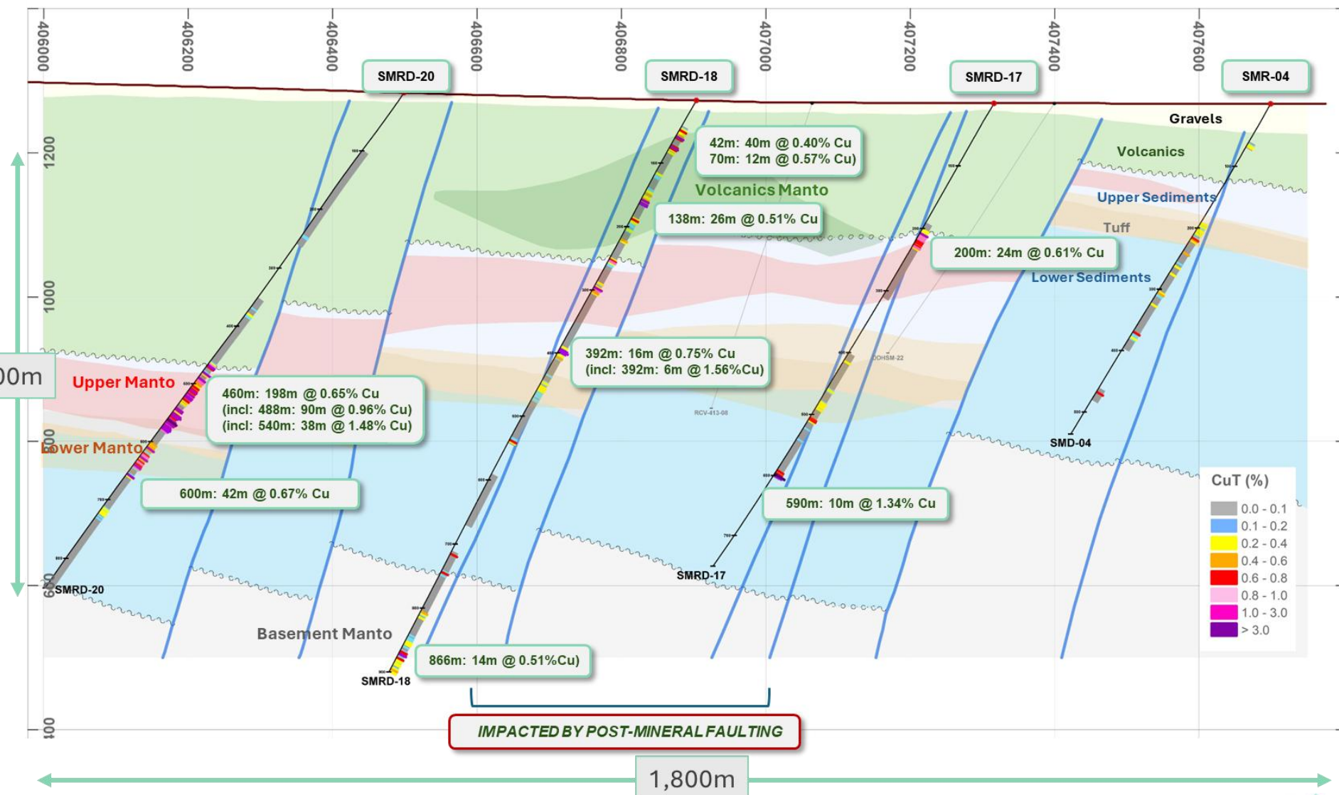
Cross Section N7441100 Looking North
