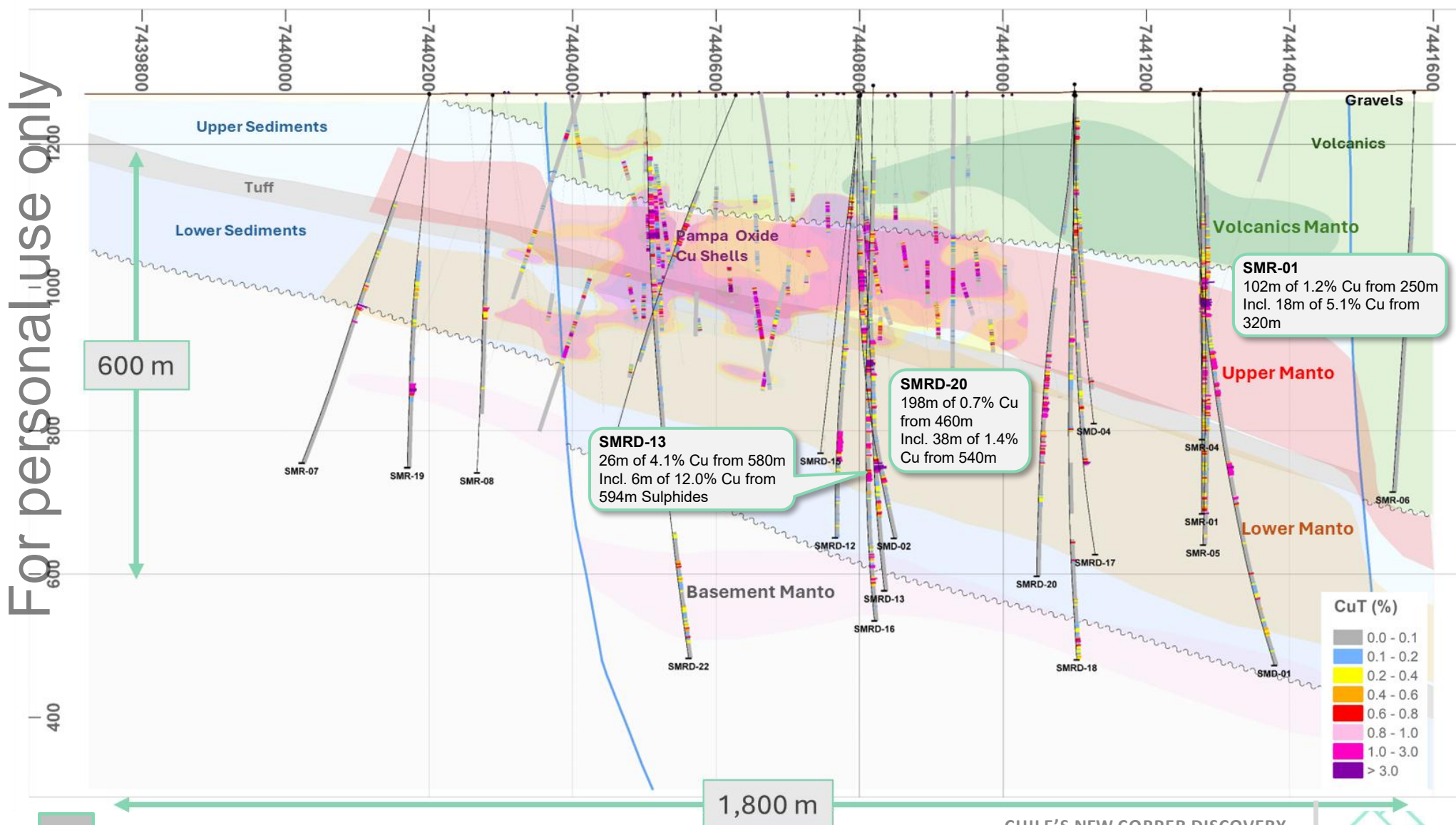
Long Section E406900 Looking West
