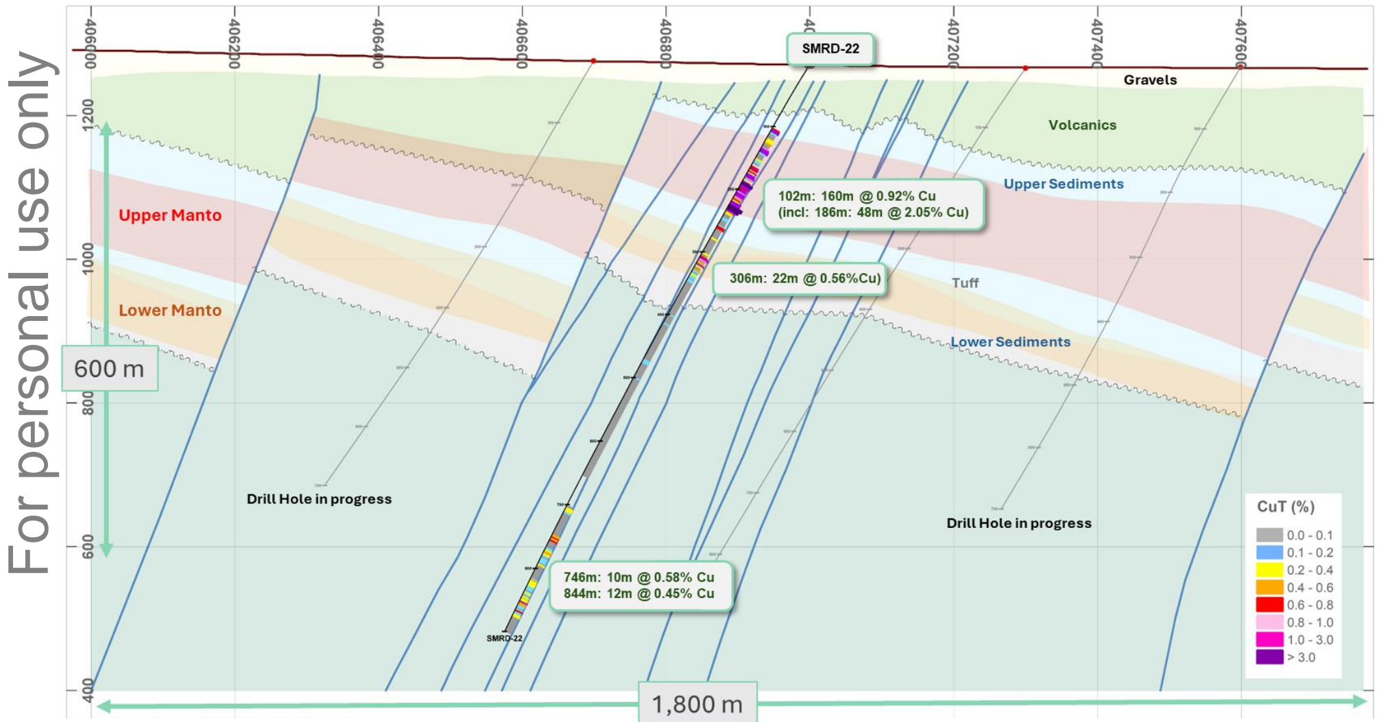
Cross Section N7440500 Looking North
