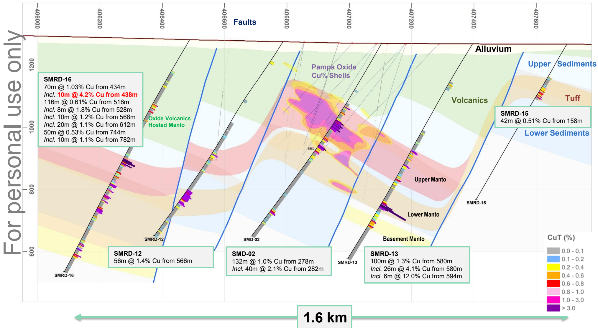
Cross Section N7440800 Looking North
