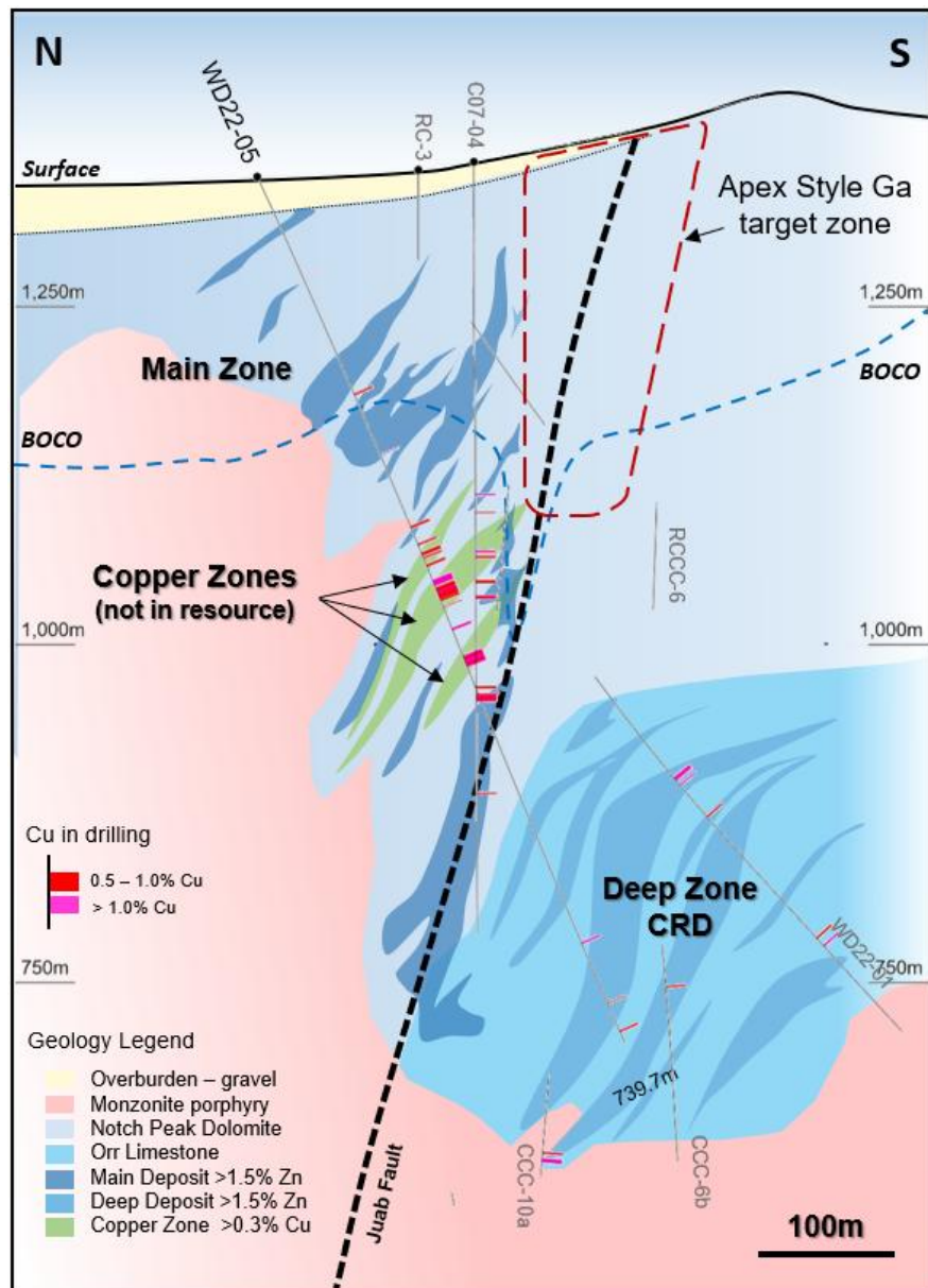
Figure 1: Section view at 288,800E (+/-20m) of the West Desert Deposit, showing existing drilling, Main and Deep Zone mineralisation, and 'Apex Mine' style gallium target area within the upper Juab Fault.
