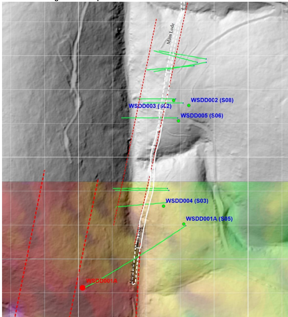
Figure3: 1 Sub-parallel mineralisation to the new West Lode.
