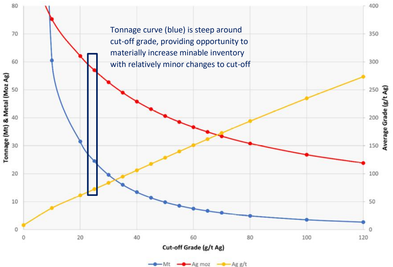
Figure 2 Paris Silver Project: Grade–Tonnage curve, Global Mineral Resource Estimate > 0mRL 1
