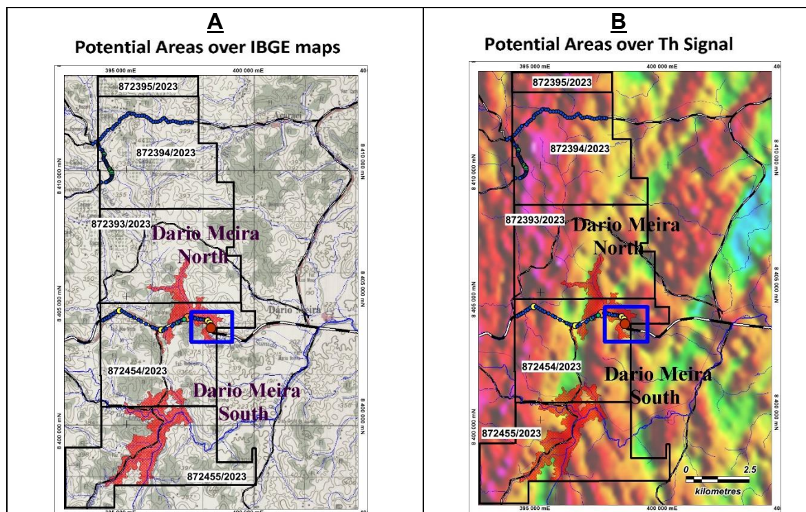
Figure 6: Jequie South - The North Dário Meira Eluvial and South Dário Meira Eluvial targets.
