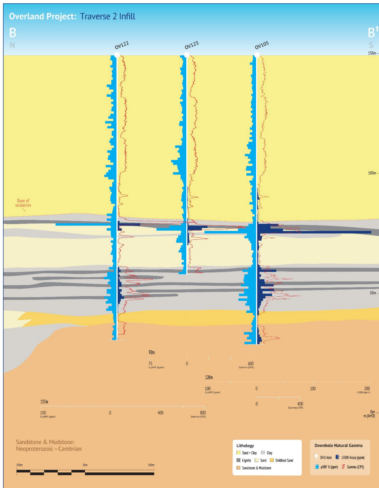
Figure 4: Infill holes OV122 (1m at 85ppm U_3O_8 from 69m), OV123 (2m at 63ppm U_3O_8 from 70m) and OV105 (1m at 213 ppm U_3O_8 from 73 m) forming part of the 300m wide anomalous zone.
