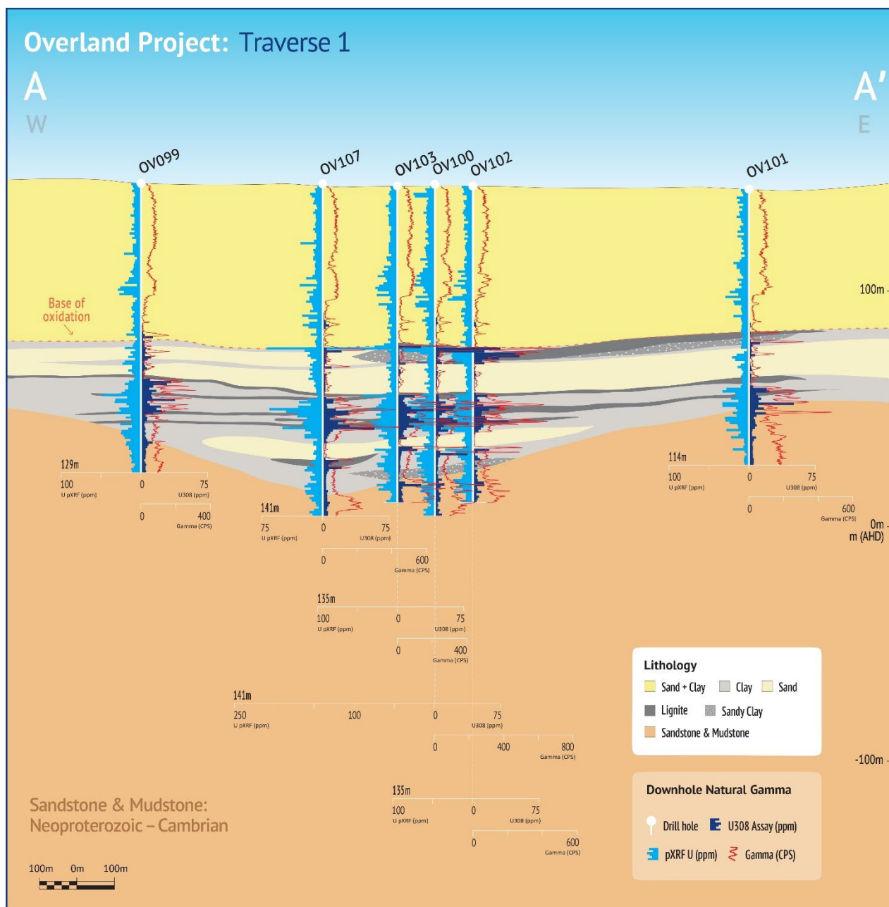
Figure 2: Cross section through OV100 (2m at 87 ppm U_3O_8 from 69m) which forms the northern extent of the 300m wide anomalous zone shown in Figure 3.
