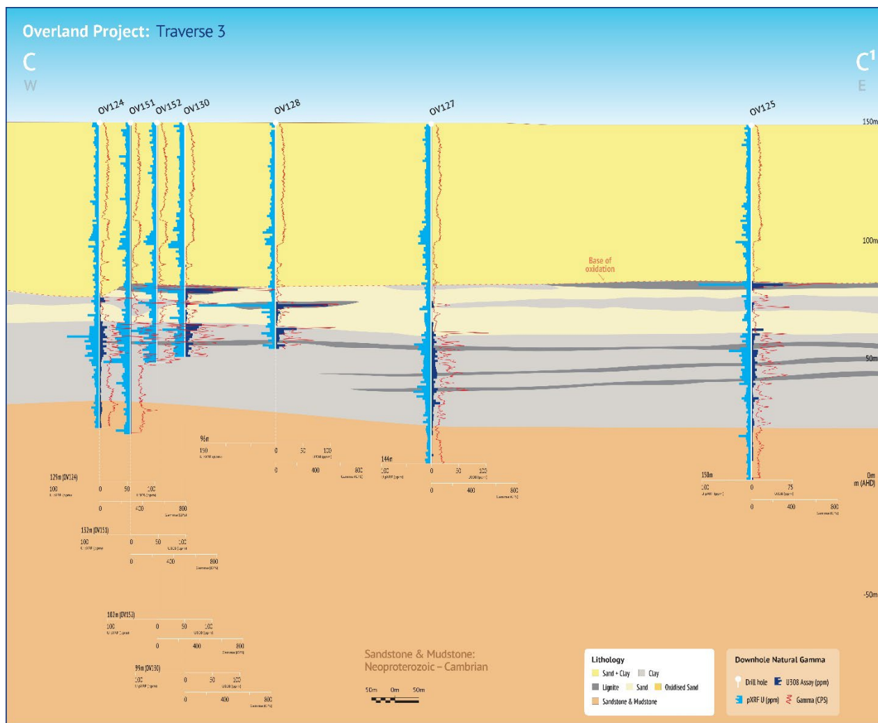
Figure 5: Section showing 200m wide anomalous zone defined by OV128 (1m at 163 ppm U_3O_8 from 77m) and OV130 (2m at 126 ppm U_3O_8 from 70m). Infill holes OV151 and OV152 contain anomalous downhole gamma through the zone with assays pending for these holes.
