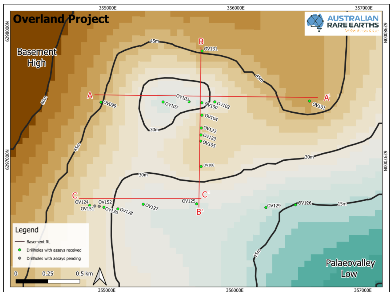
Figure 1: Overland Uranium Project – Section location plan, inset map, showing drillhole location detail for recently completed drillholes in the Northwest corner of EL7001.
