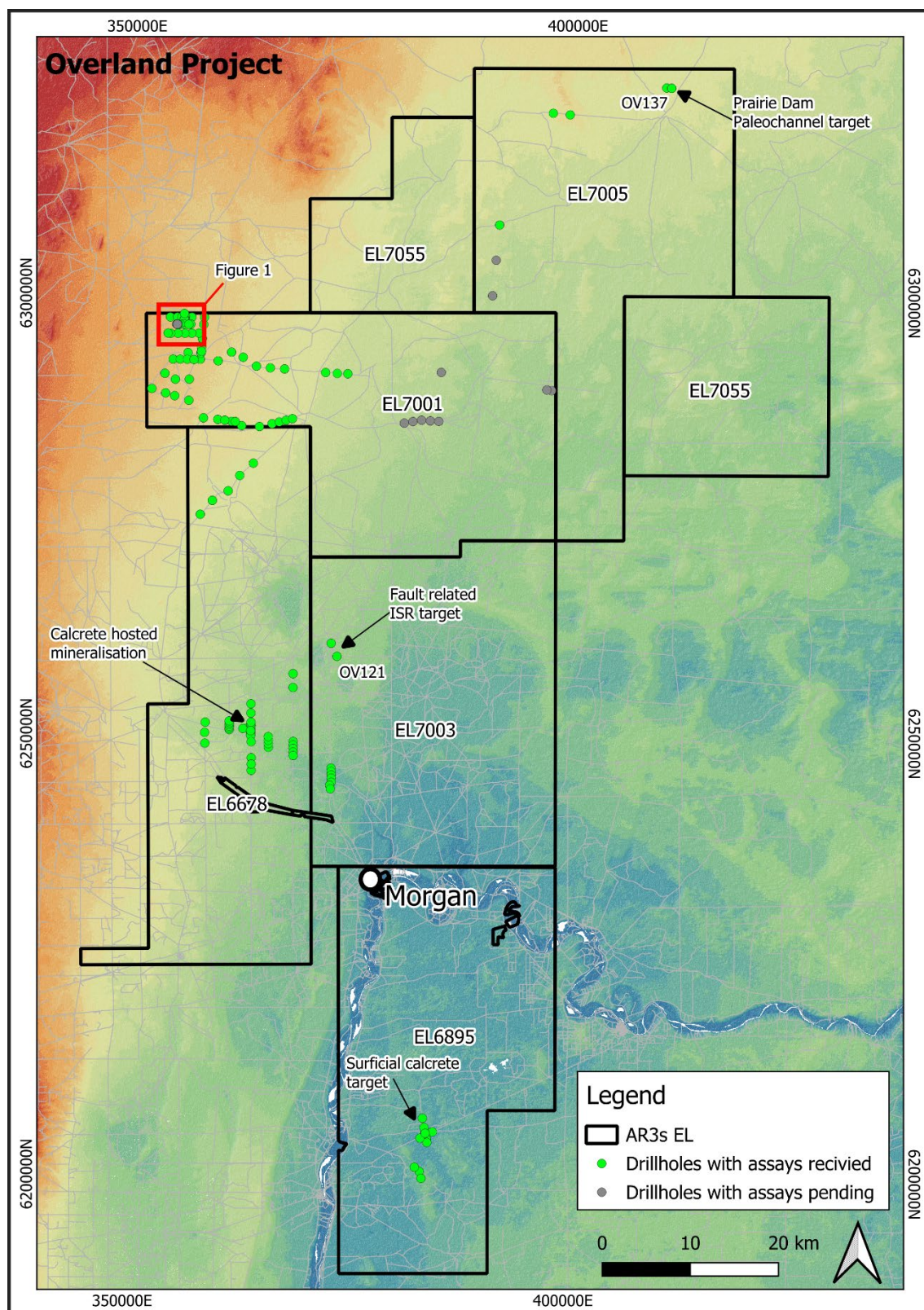
Figure 6: Overland drilling completed to date showing assays received and target areas tested with drilling
