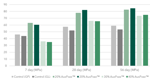
Figure 4: 40MPa Unconfined Compressive Strength (UCS)
