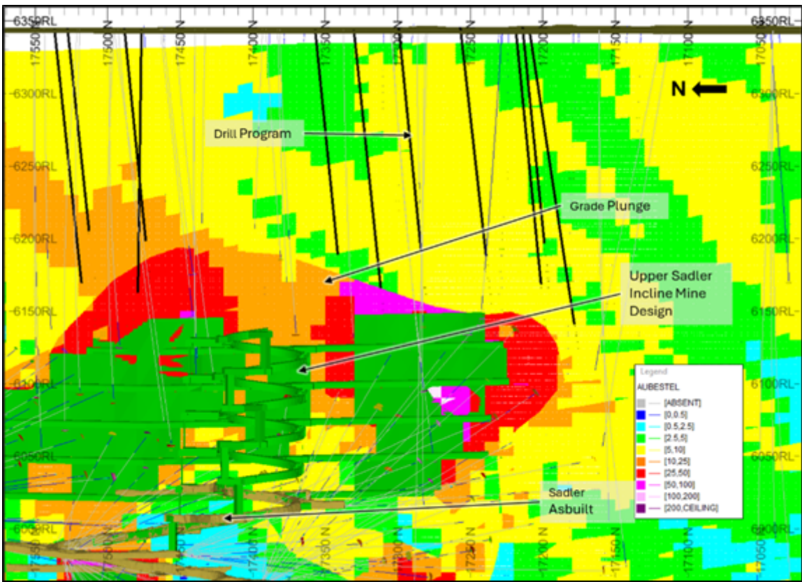
A long section view of the Upper Sadler Incline surface diamond drilling that commenced this quarter (black lines). Image shows historical drilling, Sadler As-built and planned Upper Sadler Incline Mine Design. Block model shown is the Raleigh model.
