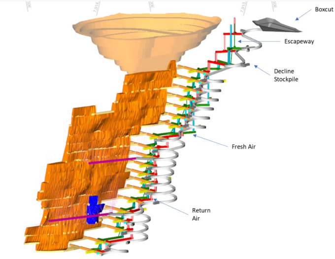
Proposed Wolverine mine layout (view looking Northeast)
