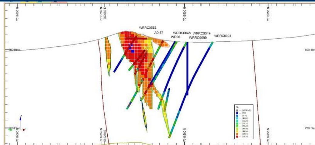
Figure 4. Madoonga section view west facing (E56500)
