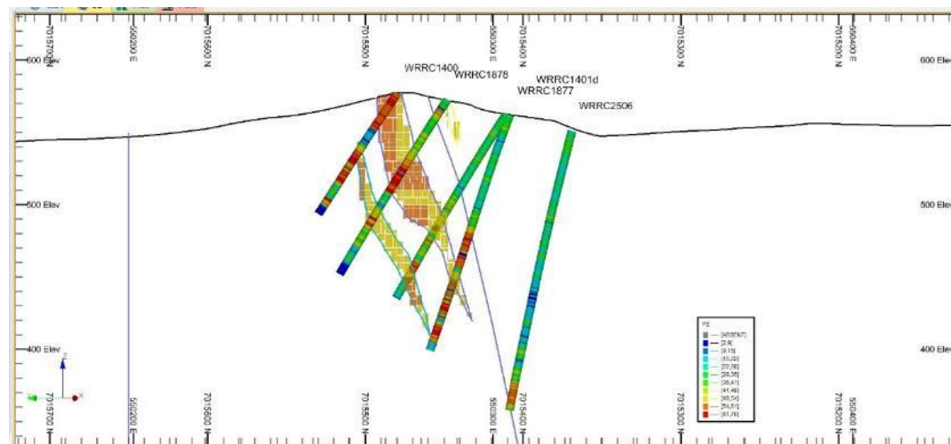
Figure 5. Madoonga West section view west facing (E550200)
