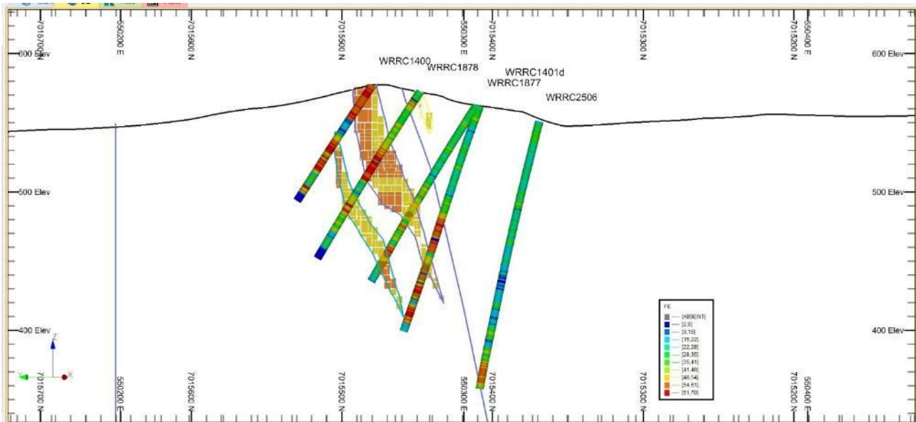
W39/39 section view north facing (N7037750)
