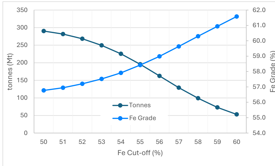
Figure 4. Weld Range Global MRE Grade-Tonnage curve
