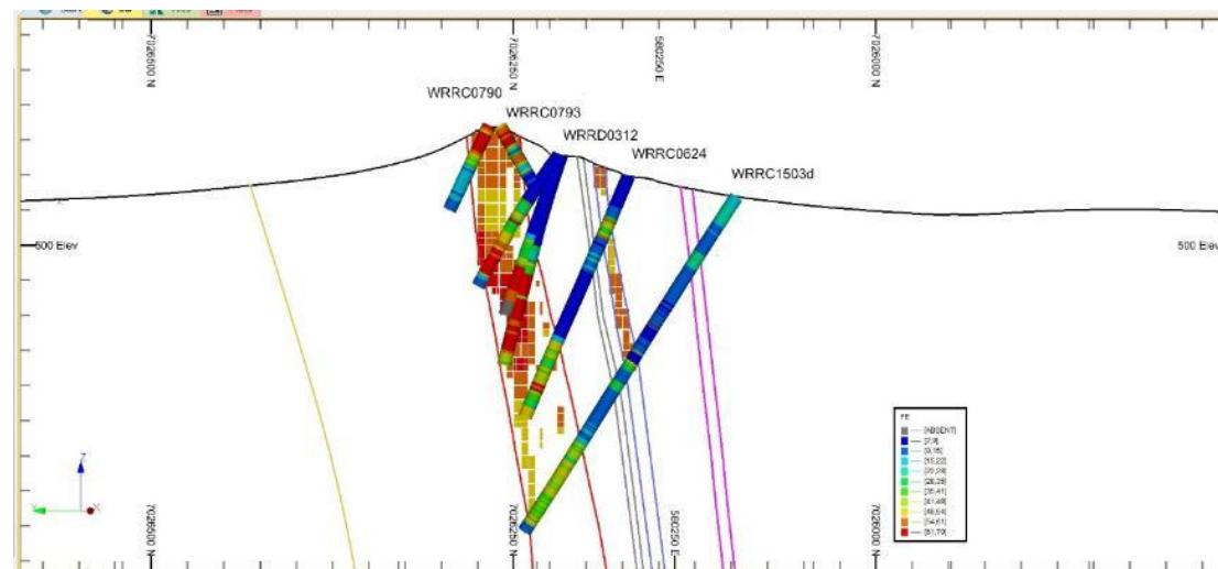
Figure 3. Beebyn North section view west facing (E68500)
