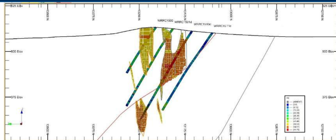
Figure 2. Beebyn section view west facing (E57900)
