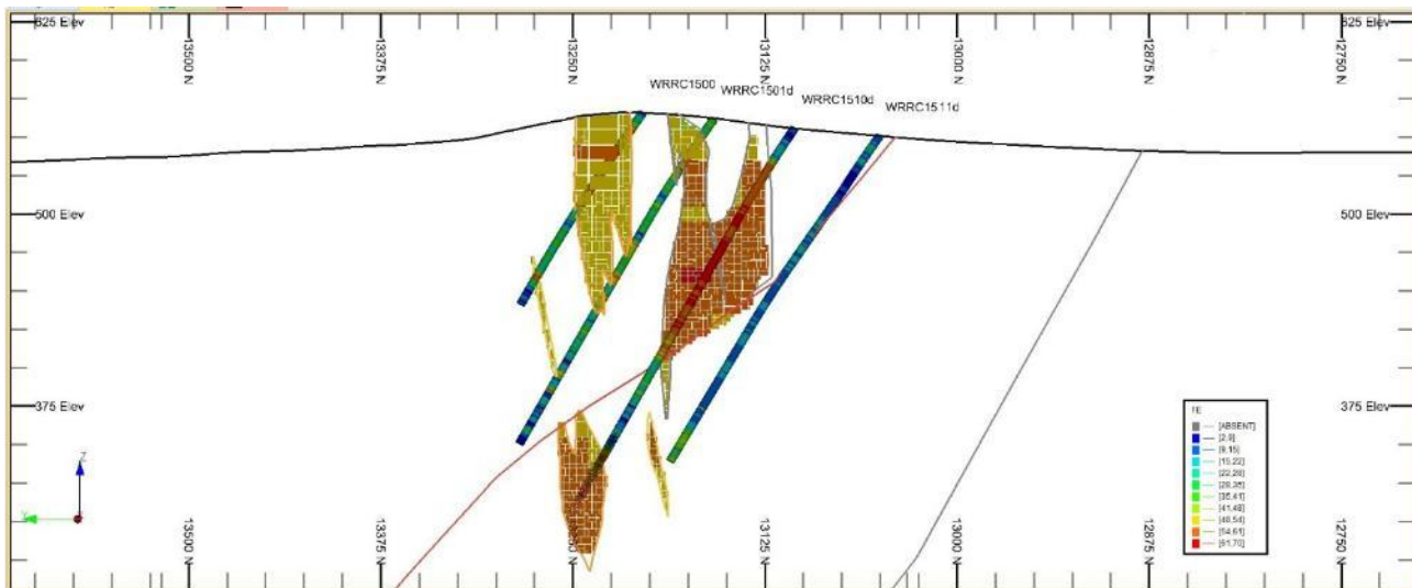
Beebyn section view west facing (E57900)
