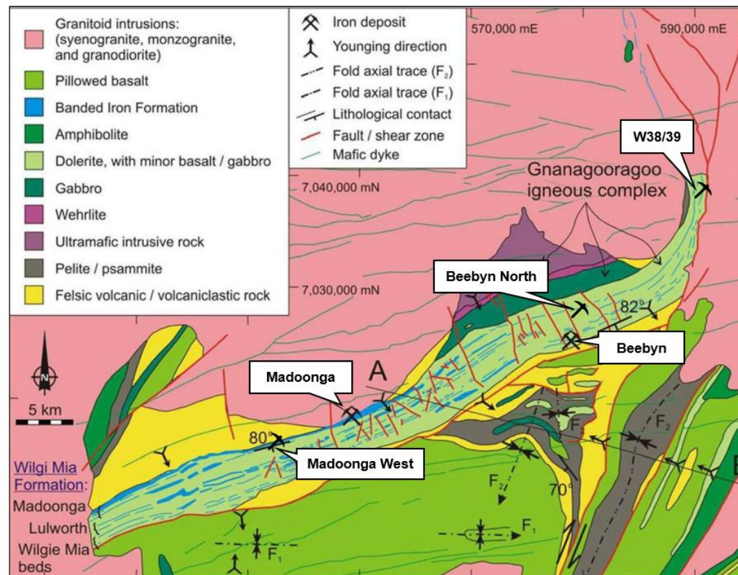
Figure 1 Geology map of the Weld Range, WA, (Duuring and Steffen, 2012)
