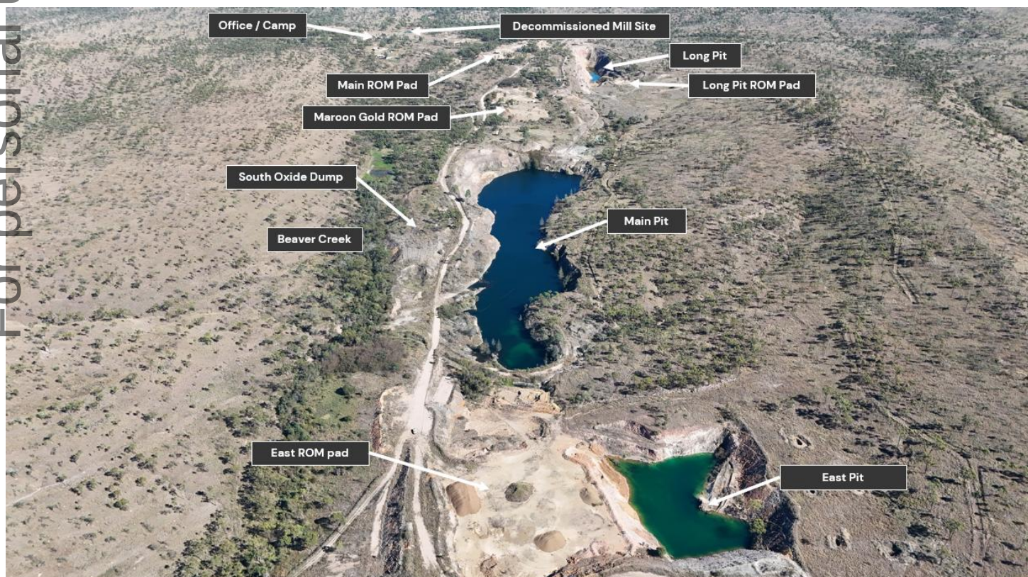
Figure 4: Aerial view of the Far Fanning Project, showing key infrastructure and open pits including the Main Pit, East Pit, Long Pit, ROM pads, and associated site facilities.
