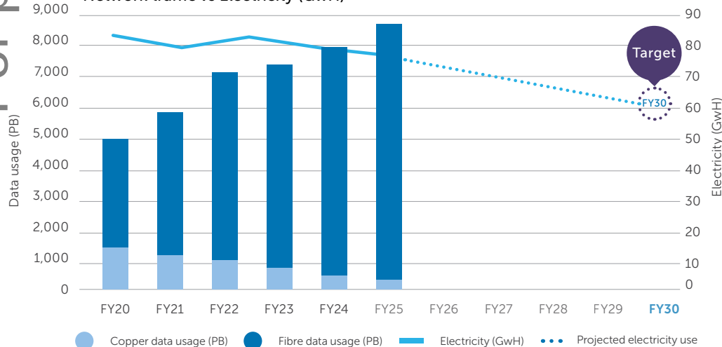
Network traffic vs Electricity (GwH)
