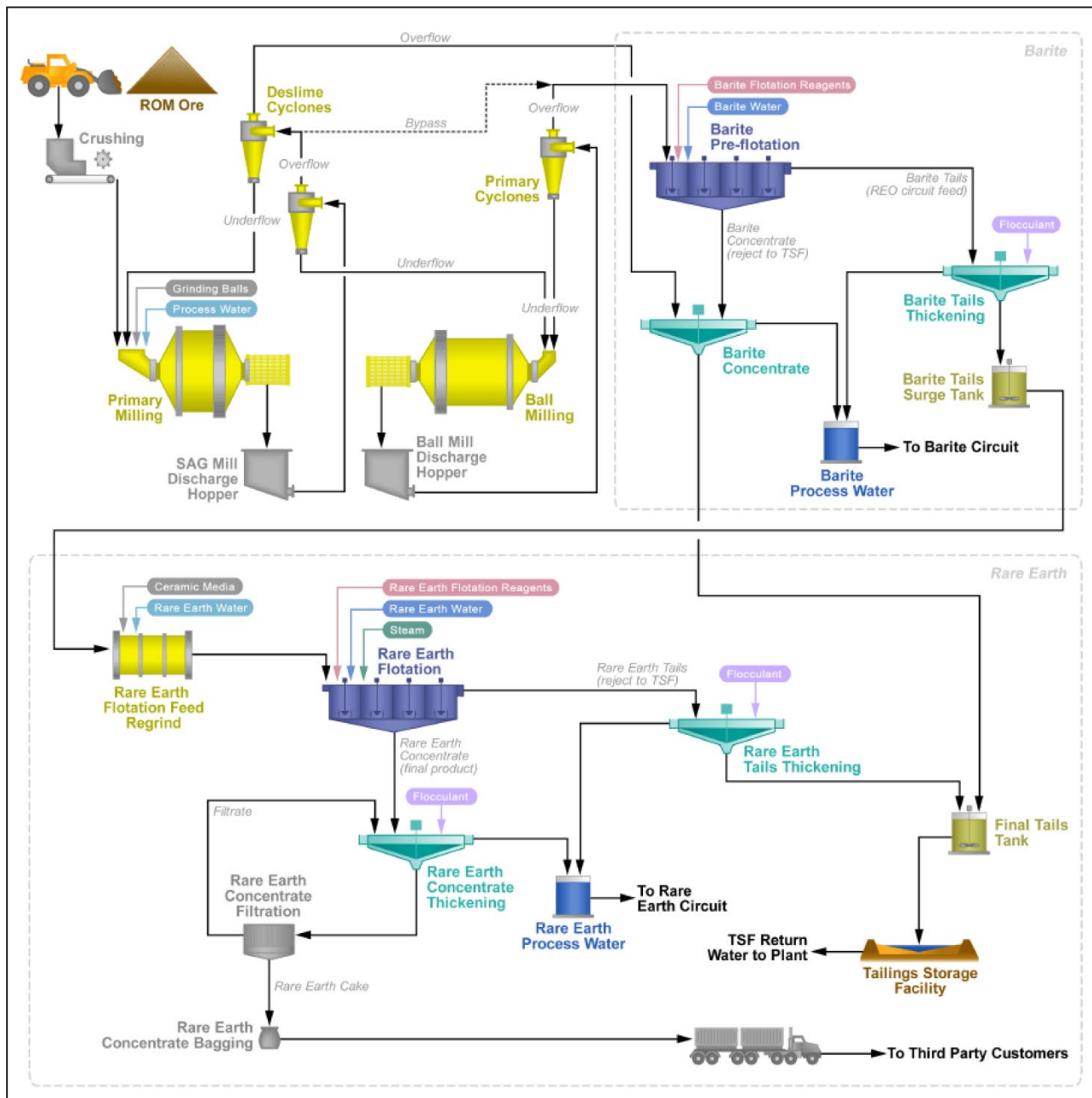
Figure 8-1: Process Flowsheet
