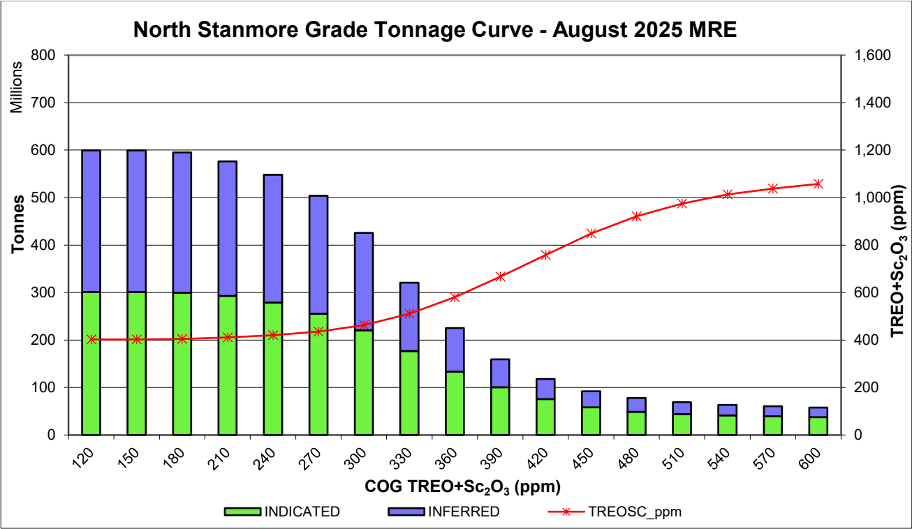
Figure 3: Grade tonnage curve for the North Stanmore TREO + Sc 2 O 3 MRE (Indicated and Inferred)
