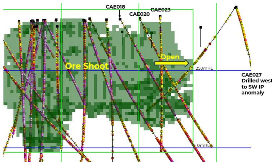
Figure 3: Long section looking due east showing the Cu ore shoot and south extension potential (0.5% Cu block model shown in green)
