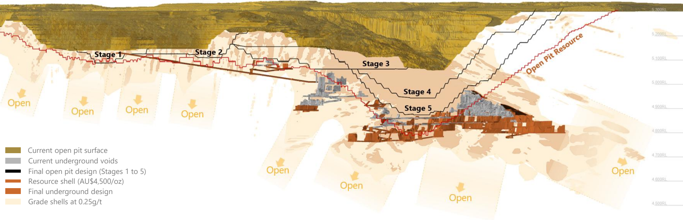
Distribution of Ore Reserve ounces within cut back stages v strip ratio
