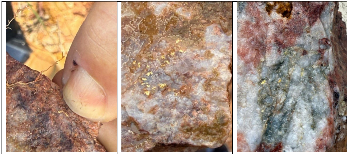
Figure 4: Visible gold observed during AUZ's site visit contained in outcrop, especially along fracture planes within brecciated quartz-sulphide veins. The ratio of visible gold to the host matrix is typically approx. 0.005% Au. These visual samples will not be sent for assaying. 6
