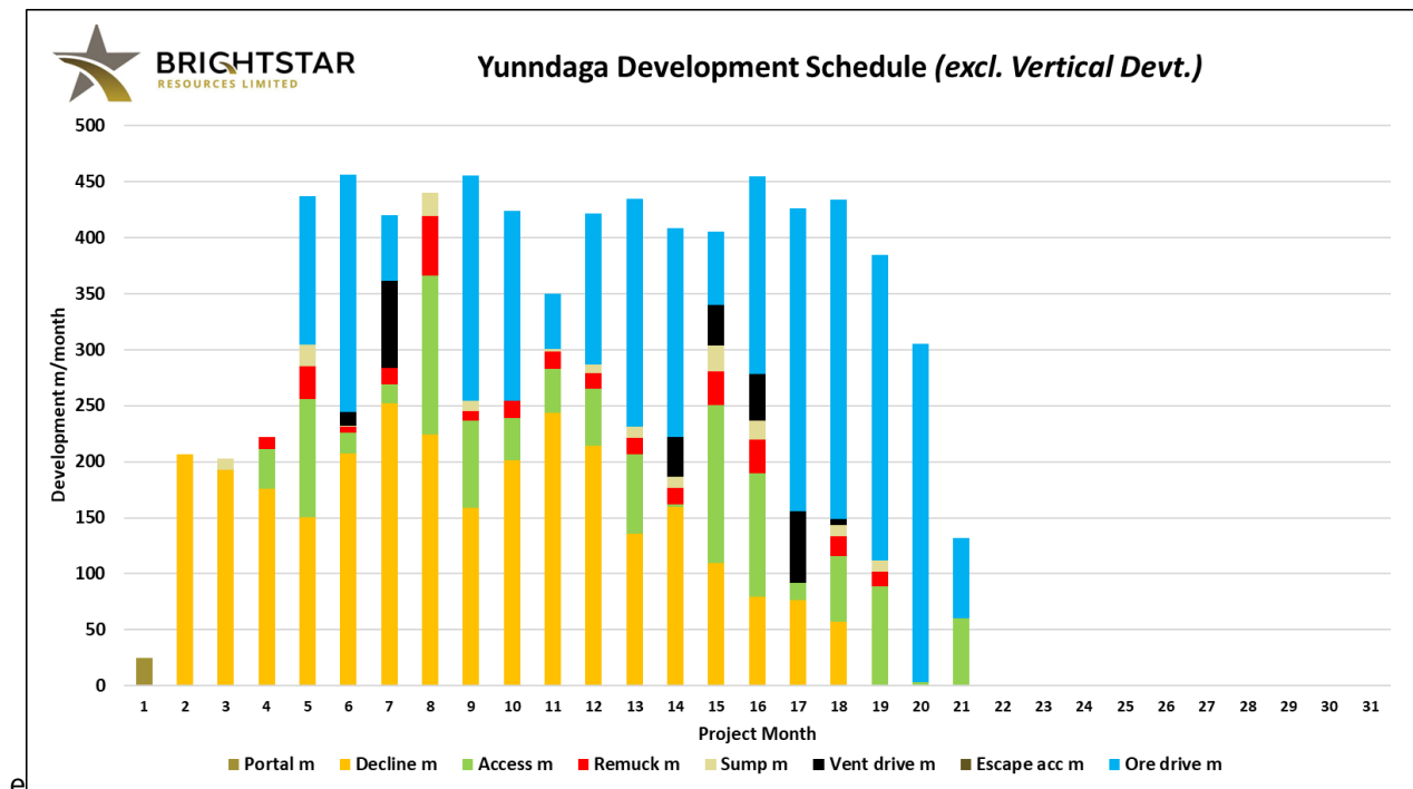
Figure 36: Yunndaga UG conceptual development schedule
