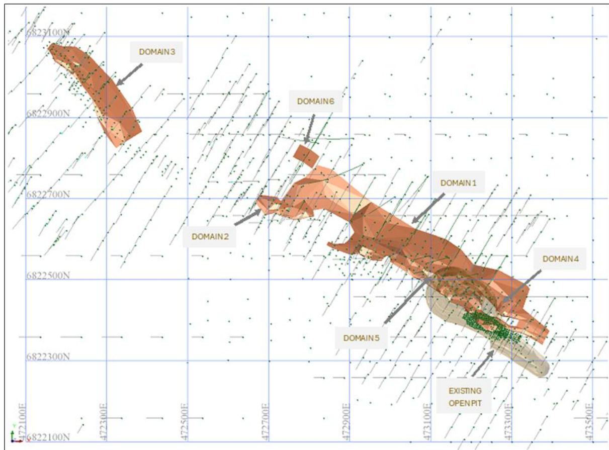
Figure 70: Plan view of Alpha Mineralised intercepts
