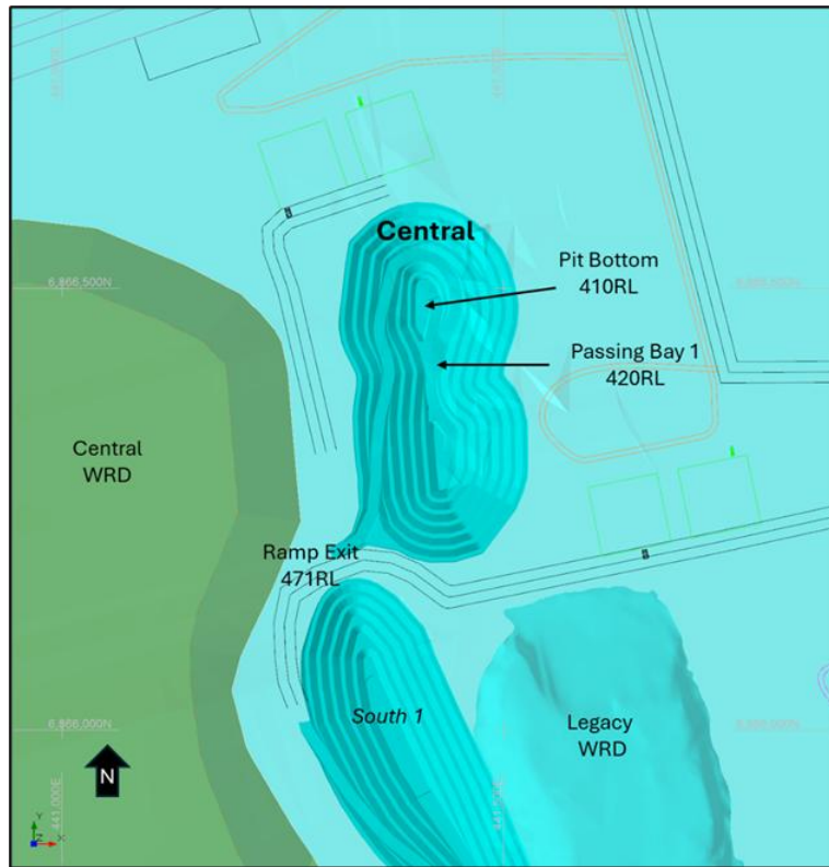
Figure 25: Plan view – Cork Tree Well (Central) pit design
