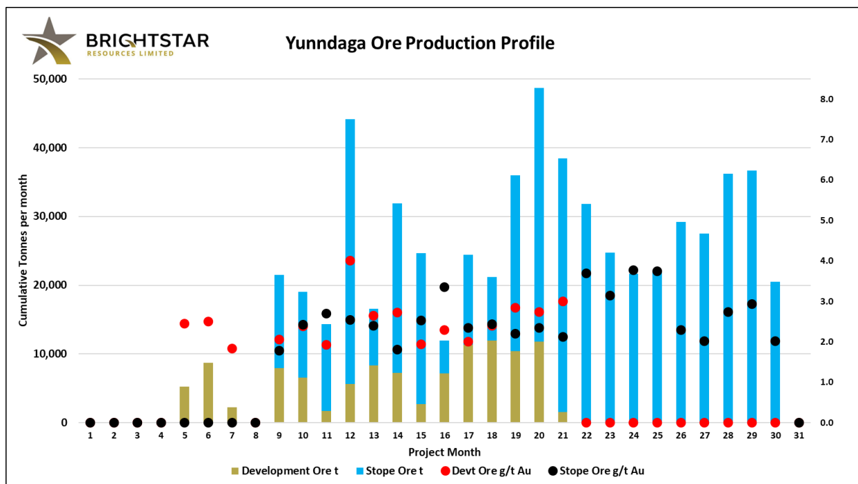
Figure 37: Yunndaga UG conceptual ore production profile
