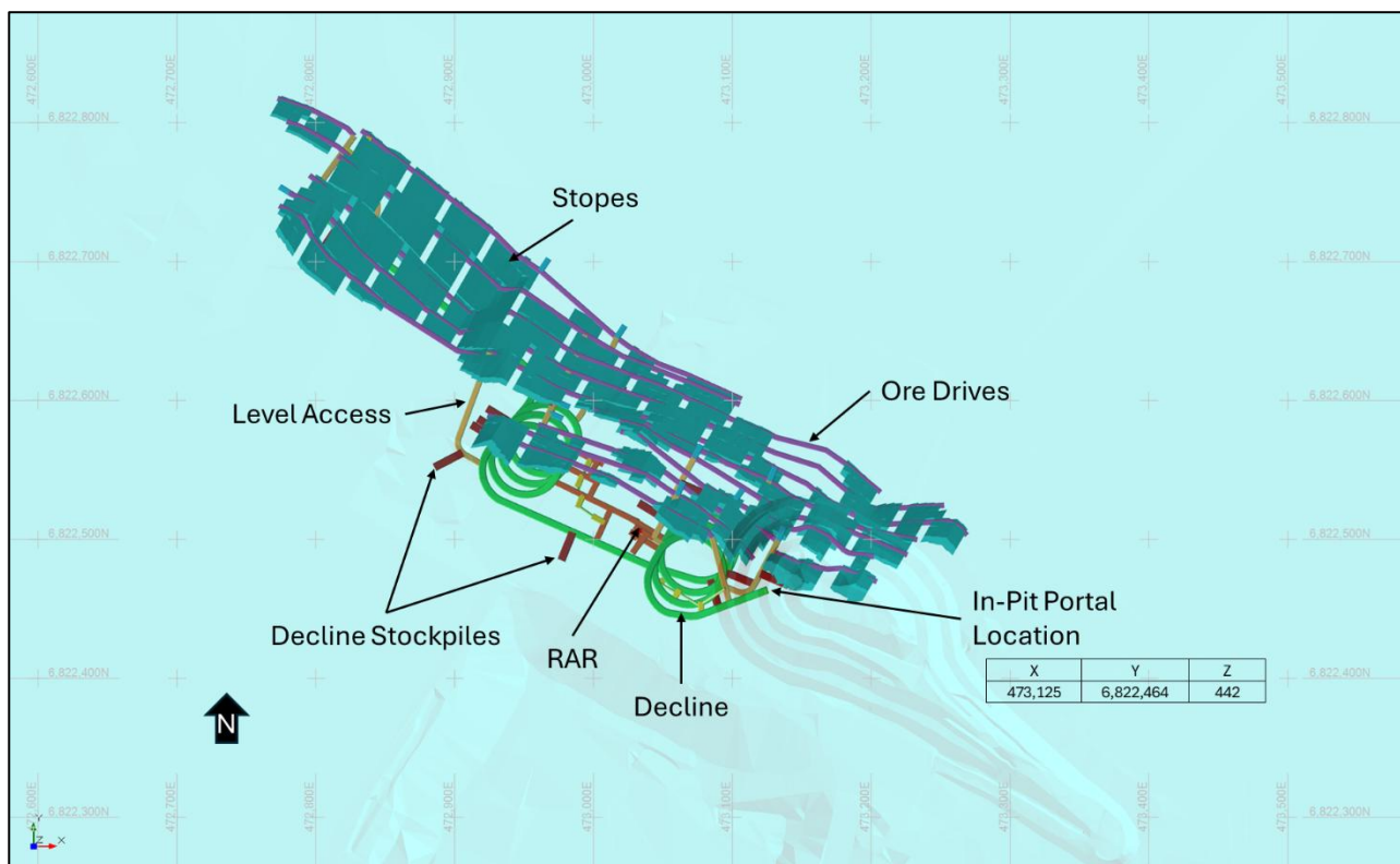
Figure 33: Alpha UG concept design (plan view)
