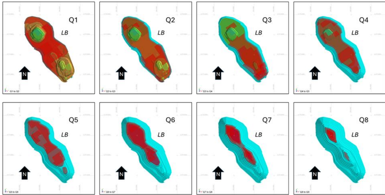
Figure 49: Plan view of Lord Byron – Ore Reserve schedule by quarters
