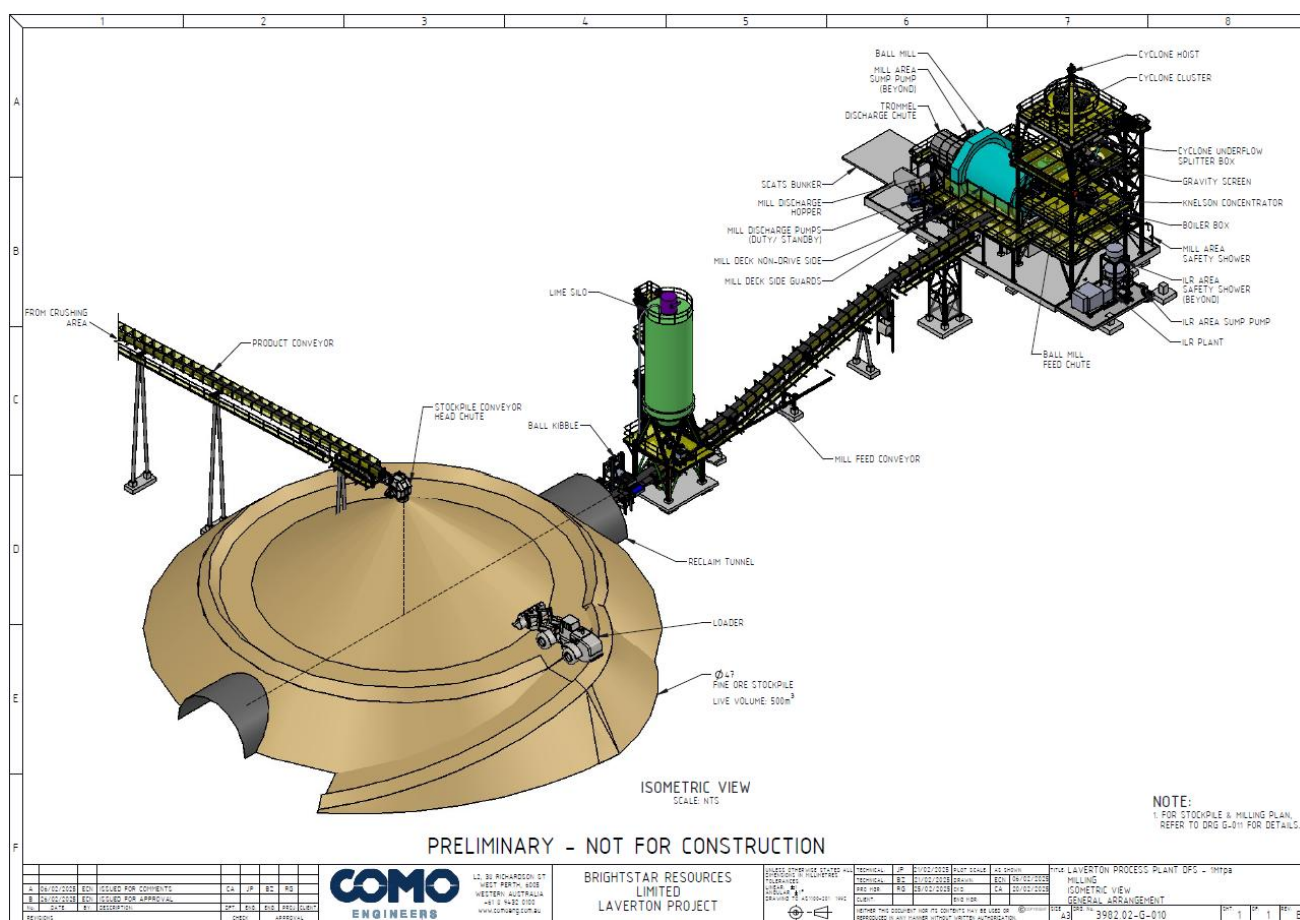
Figure 60: Oblique view of Beta milling circuit (Como, 2025)
