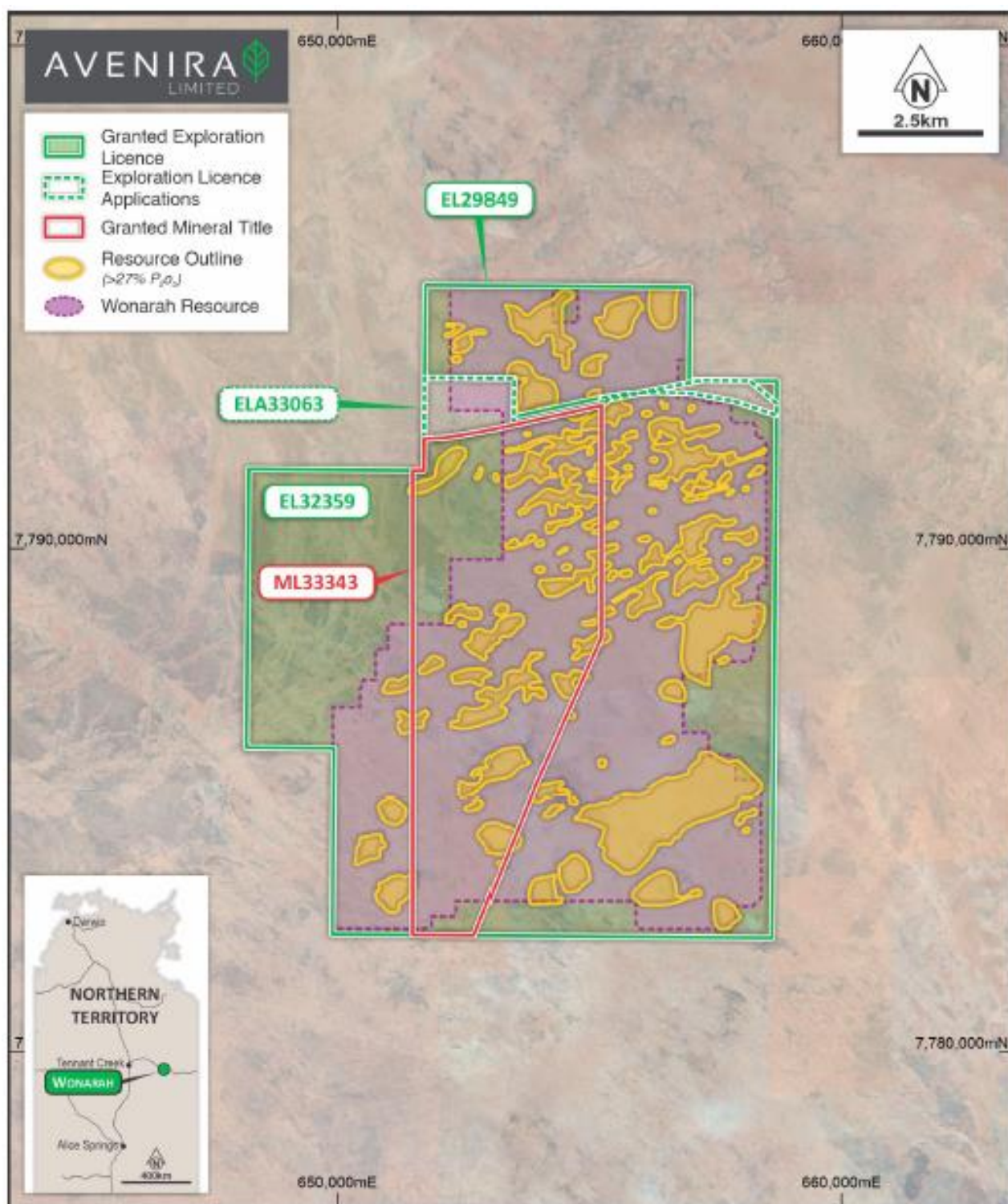
Figure 4-9: Wonarah Main Zone Resource Block Model >27% P 2 O 5 .
