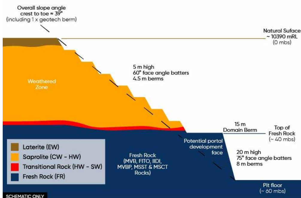
Figure 5.7: GBE Pit Wall Design Parameters
