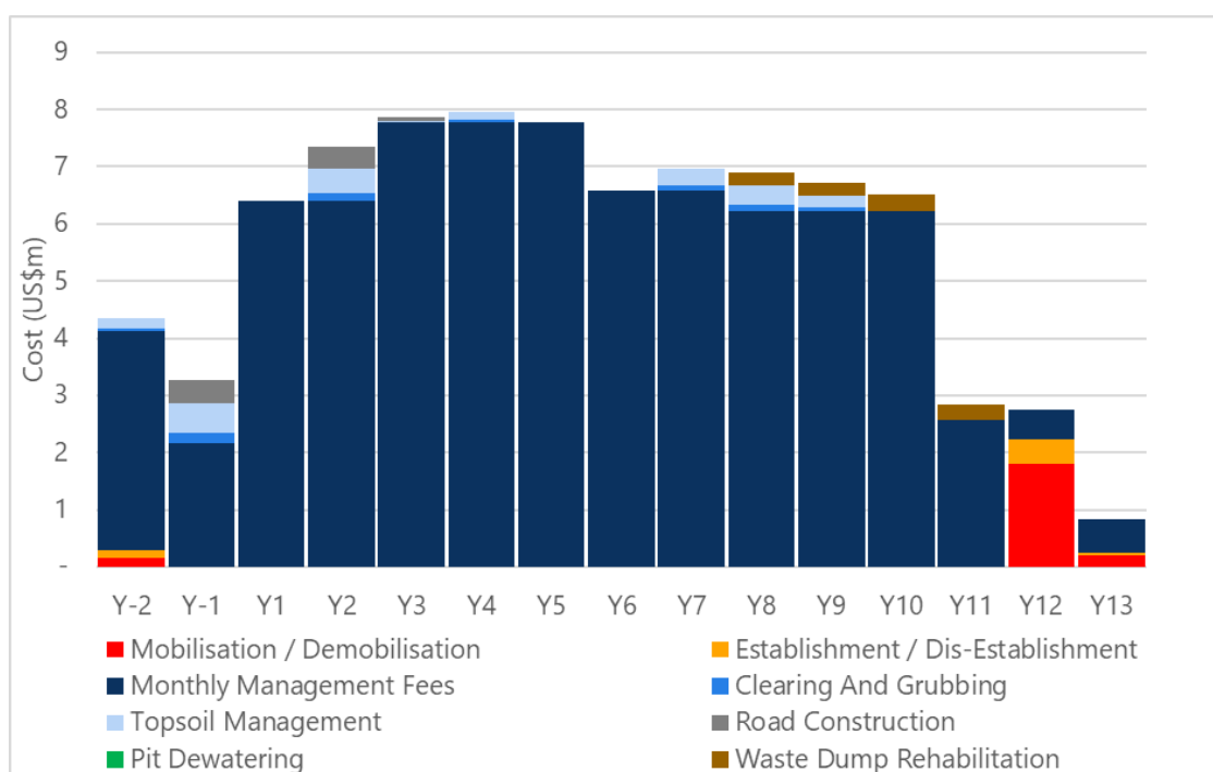
Figure 16.1: Fixed Open Pit Contractor Costs over LOM
