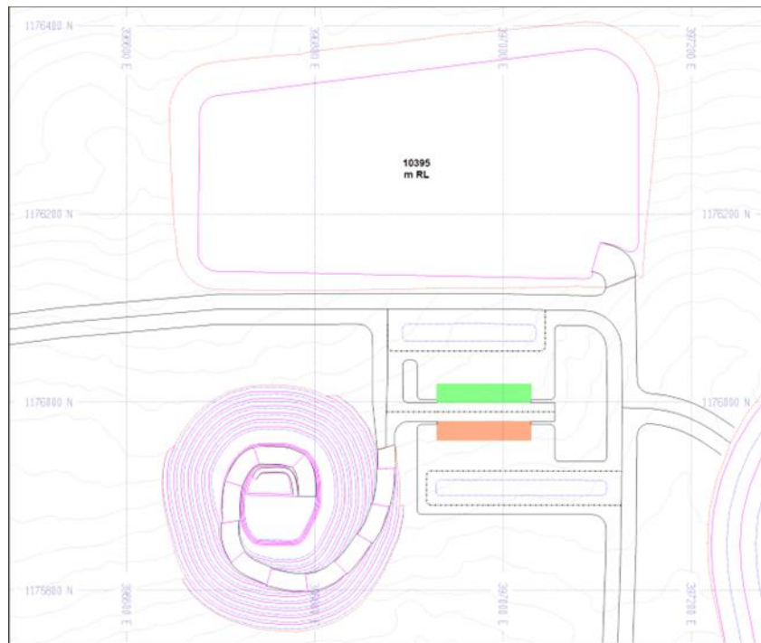
Figure 8.9: GBE Waste Rock Dump Layout
