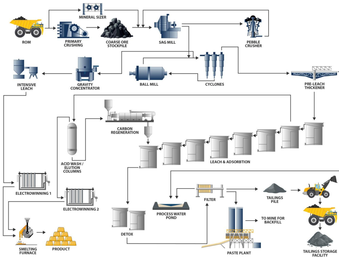
Figure 9.1: Process Flowsheet
