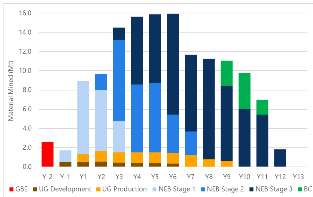
Figure 8.24: Life of Mine Schedule – Total Material Mined
