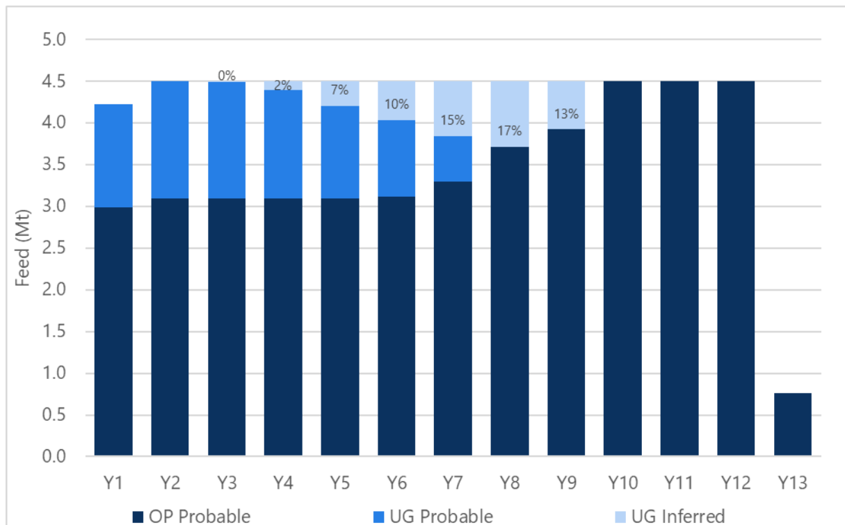
Figure 8.26: Life of Mine Schedule – Mill Feed Tonnes by Mineral Resource Classification
