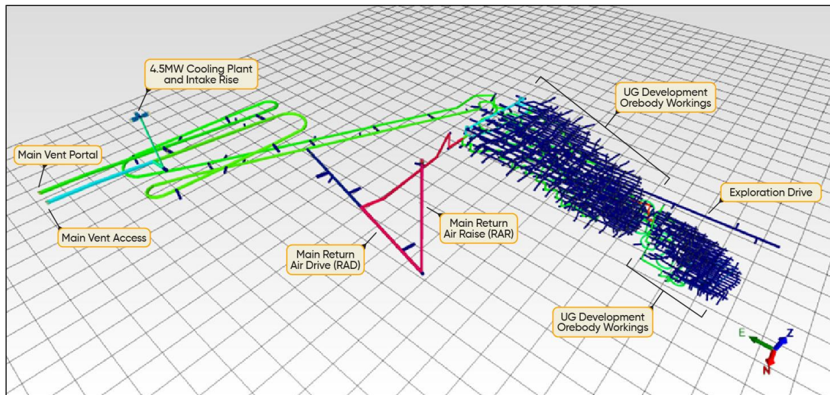
Figure 8.16: Mine Ventilation Circuit (from Ventsim® Software)
