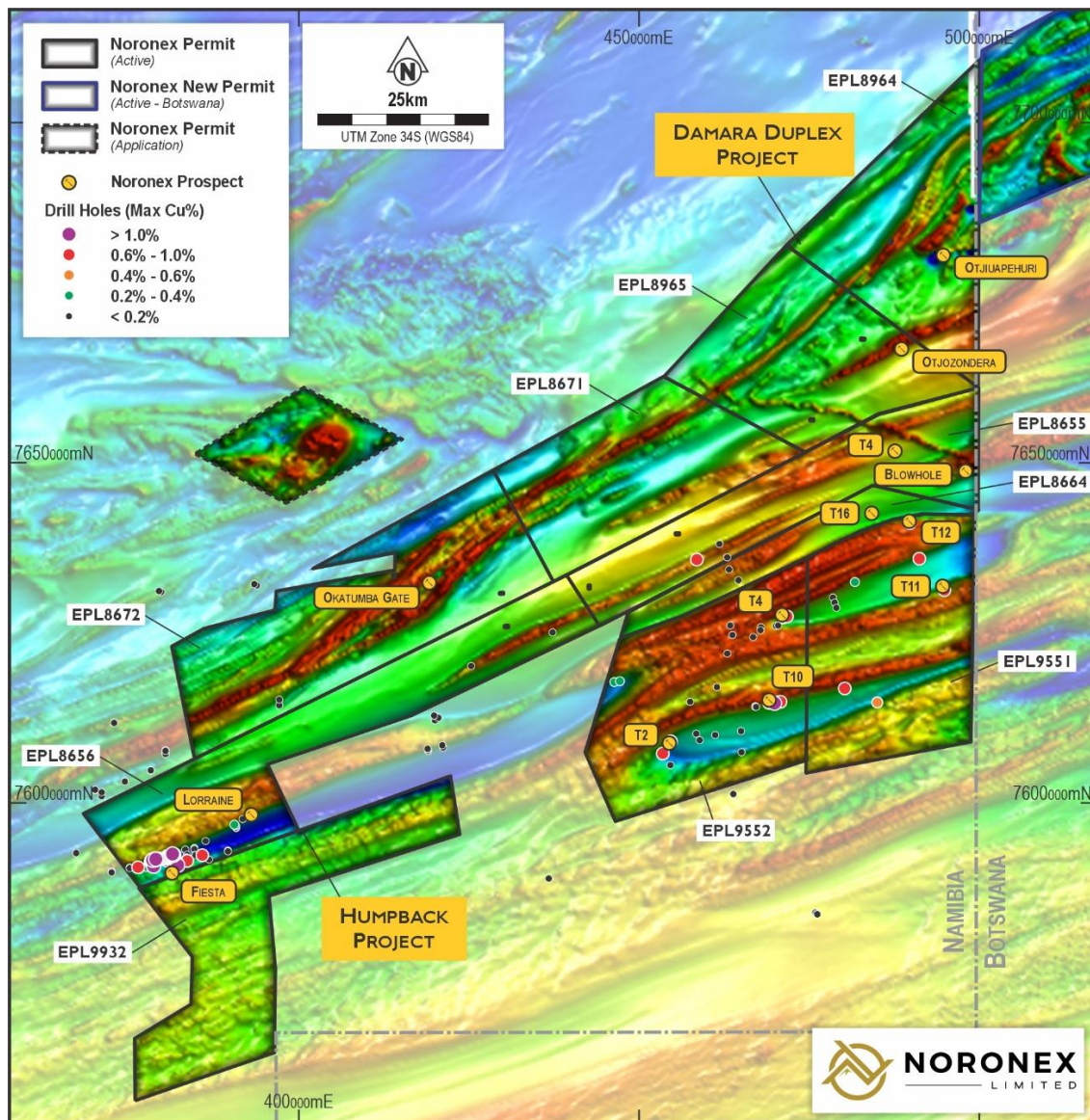
Figure 2: Regional aeromagnetic image of the Kalahari Copper Belt in Namibia with the current Noronex projects showing Fiesta in the west and a number of magnetic complexes in the north of Damara
