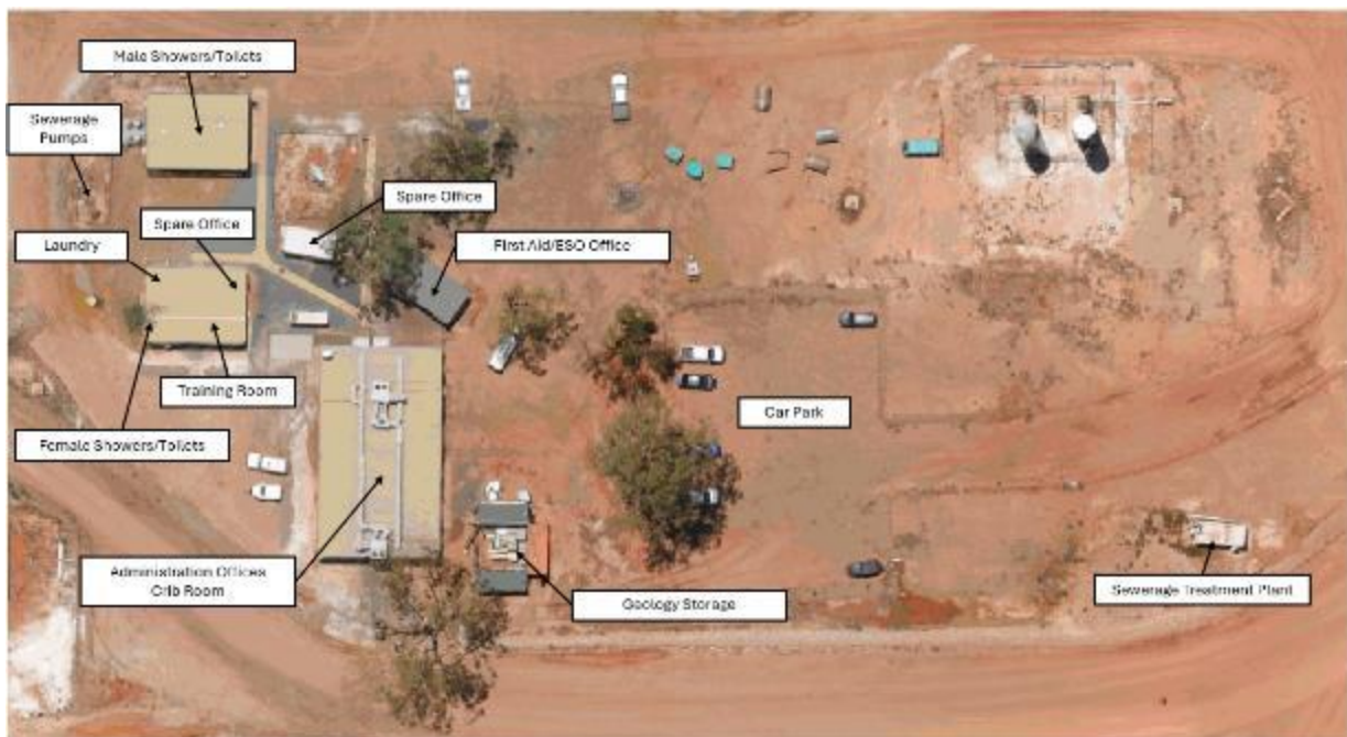
Figure A16: Layout of the existing administration and abluion facilities
