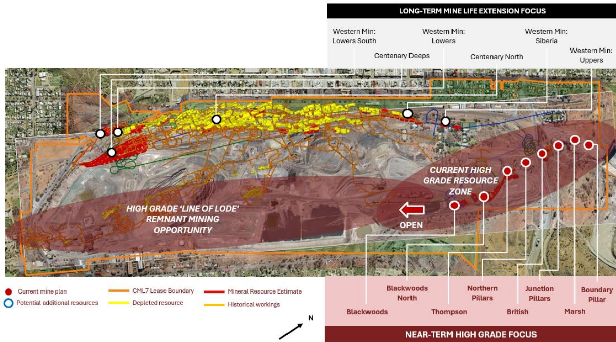
Figure 3 - Plan view of the Rasp Mine
