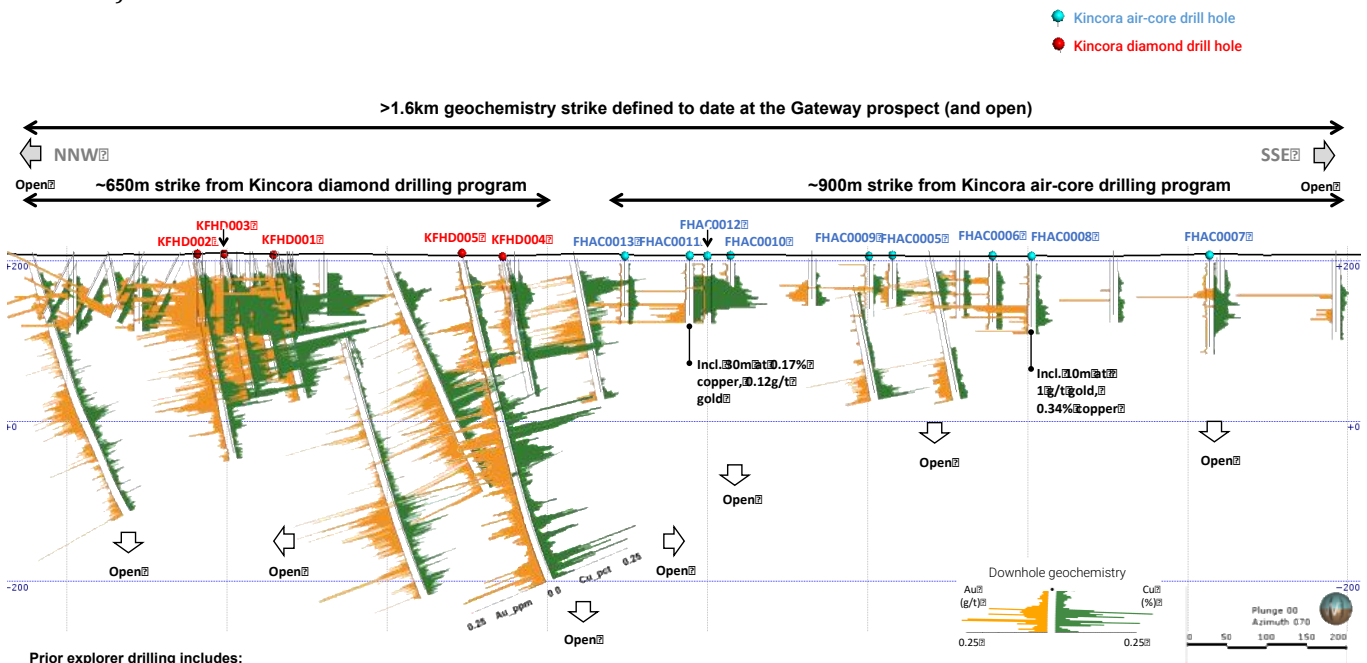
Figure 12: Gateway long section illustrates extensive mineralised system largely untested at depth and open Long section to Figure 11
