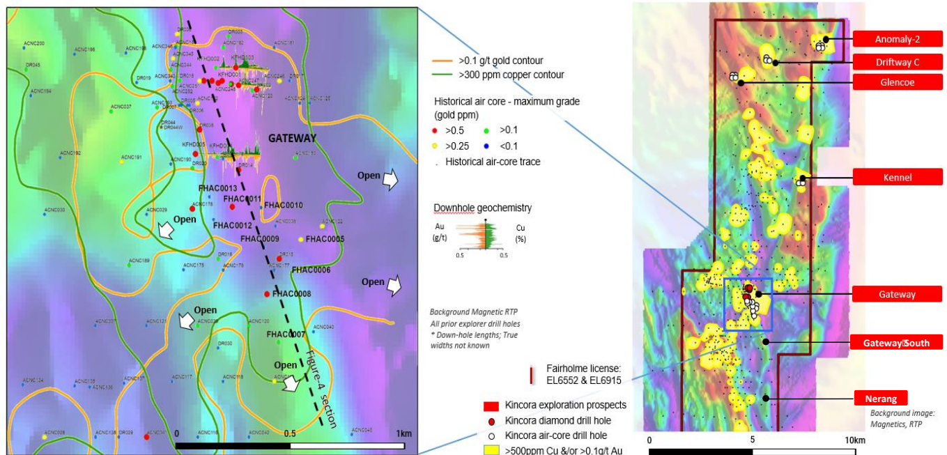
Figure 11: Gateway prospect strike >1.6km with vectors (long section Figure 12)
