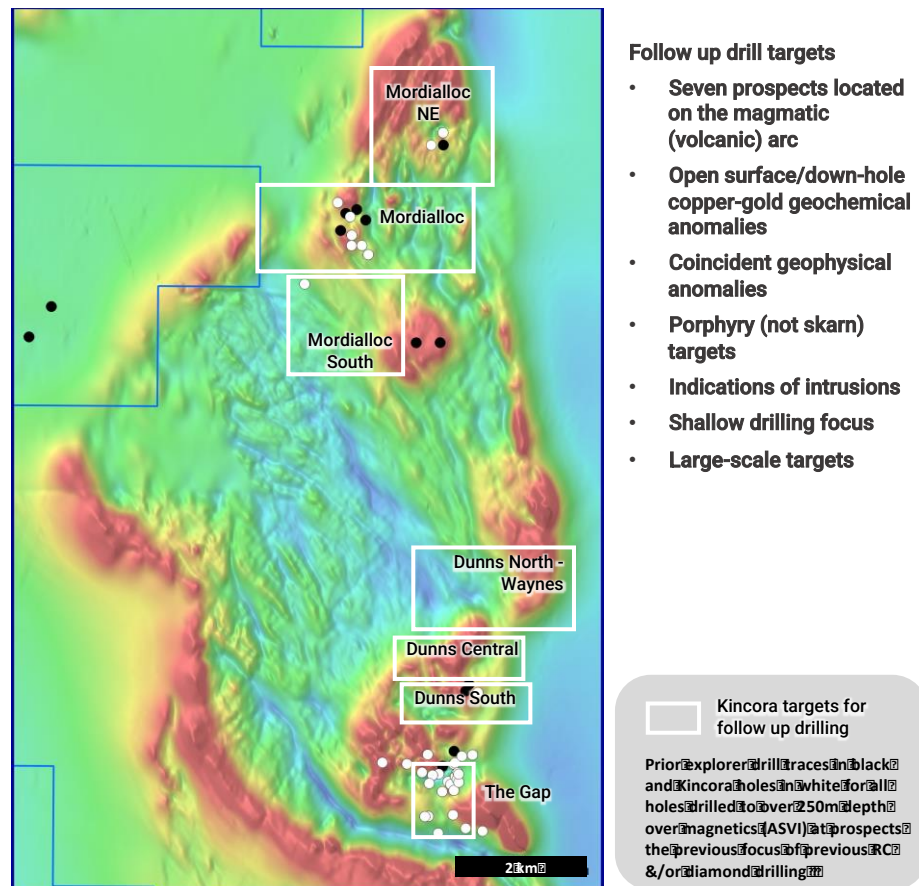
Figure 19: Seven large-scale, separate porphyry prospects identified for follow up drilling In December 2023, Kincora consolidated a 100% interest in the Trundle project
