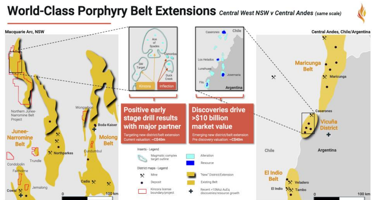
Figure 5: Macquarie Arc v Central Andes (same scale). Kincora’s NJNB portfolio (including the total AngloGold Ashanti earn-in and Kincora wholly owned licenses) now covers a strike length that is twice that of the rapidly emerging Vicuña porphyry district Kincora’s NJNB portfolio (including the total AngloGold Ashanti earn-in and Kincora wholly owned licenses) now covers a strike length that is twice that of the rapidly emerging Vicuña porphyry district.
