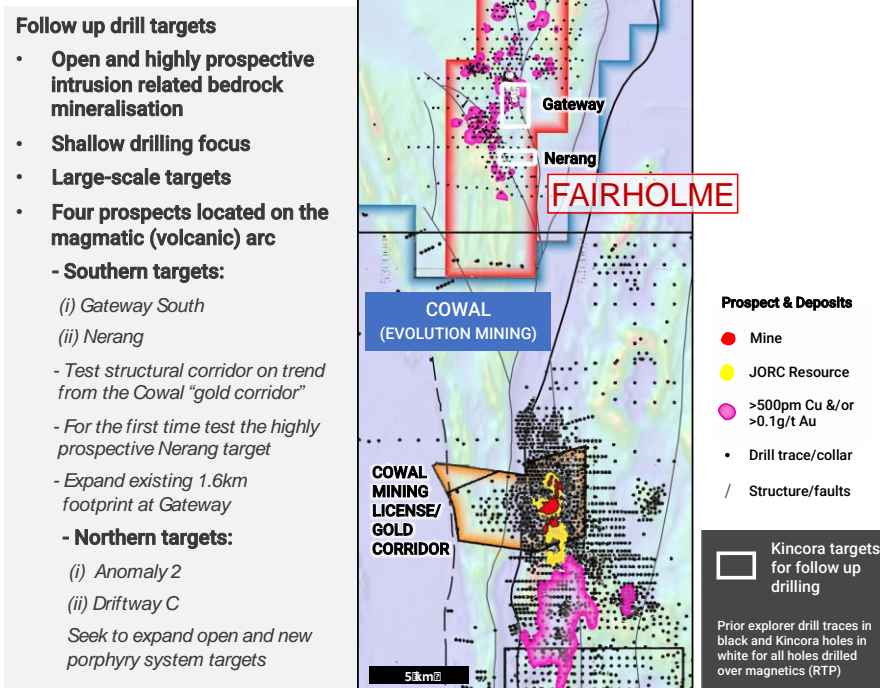
Figure 14: Four large-scale prospects identified for follow up drilling
