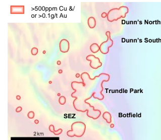
Figure 17: The Trundle projects hosts large mineral systems in the north and south of the license, comparable in scale to the existing mine and earn-in partner exploration projects in the immediate district
