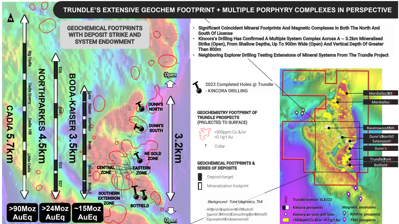
Figure 18: Kincora 2023 drilling at Trundle has confirmed an extensive multiple system gold-copper complex
