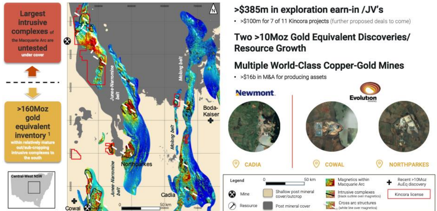
Figure 4: Magnetics maps Macquarie Arc volcanic belts, intrusive complexes and mineralised systems
