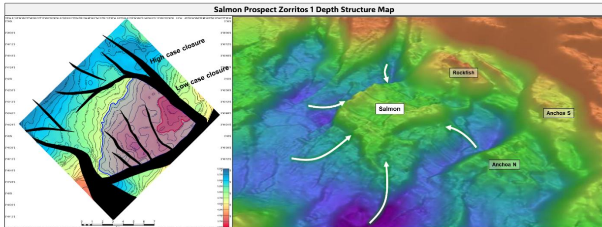
Figure 7 – Salmon prospect Zorritos 1 depth map and perspective view.
