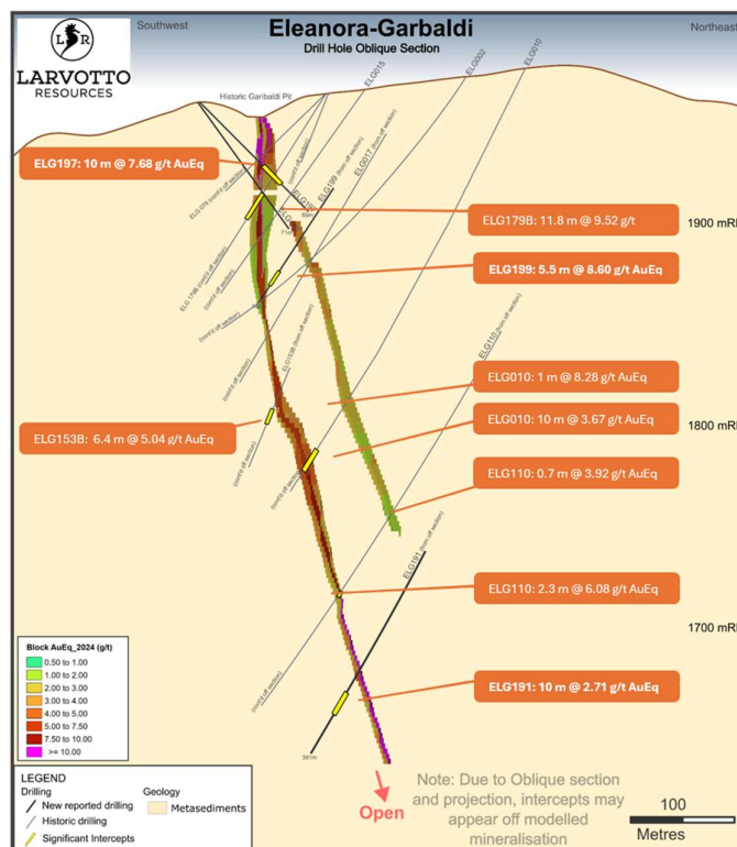
Figure 5. Garibaldi Cross Section
