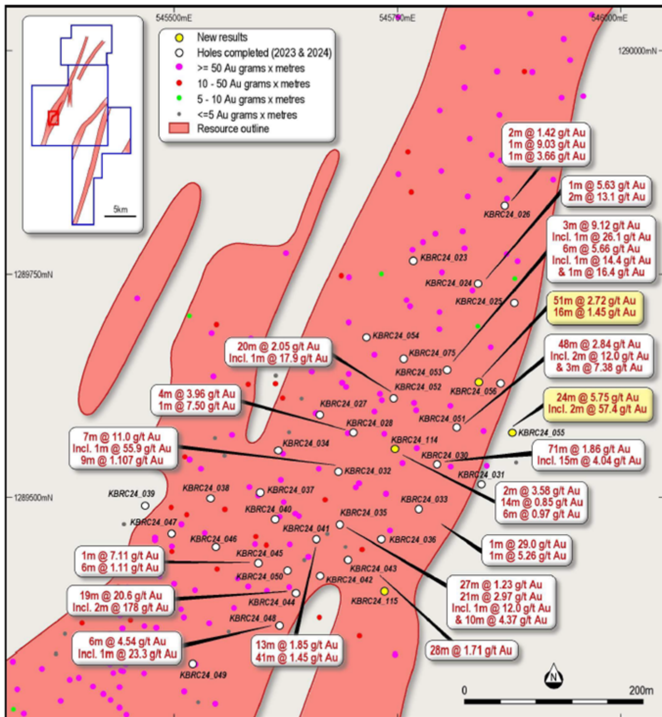
Figure 1: Results received from resource definition drilling at the Kobada Gold Deposit - Central Area
