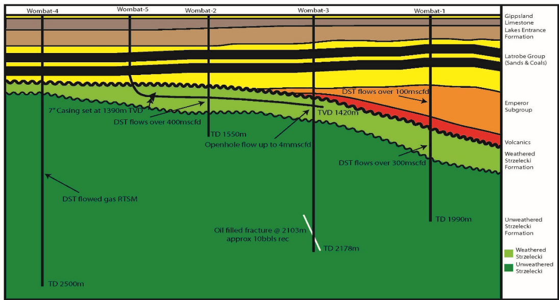
Figure 2: Cross-section of Wombat-5 Gas Well
