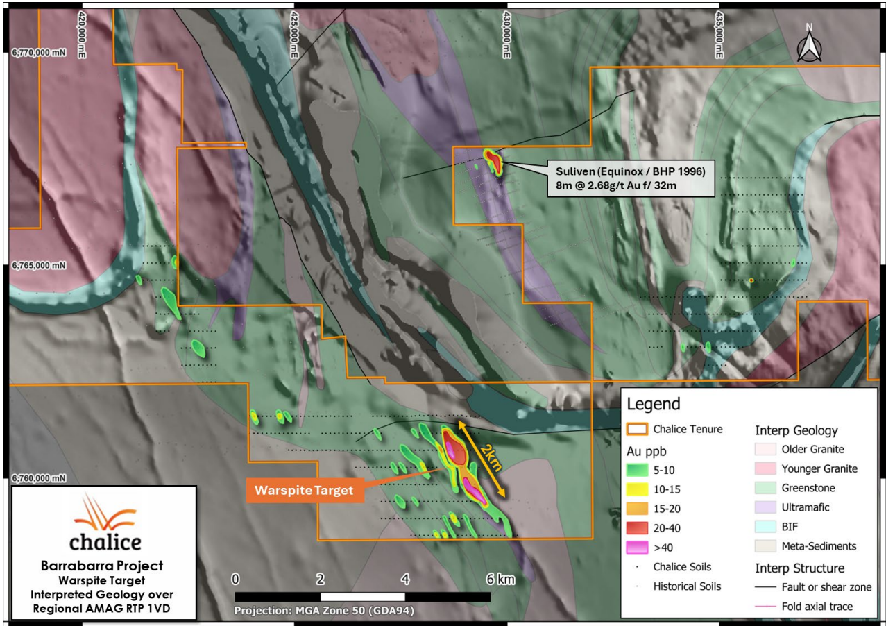
Figure 5. Warspite and Suliven Targets, interpreted geology over aeromagnetics.
