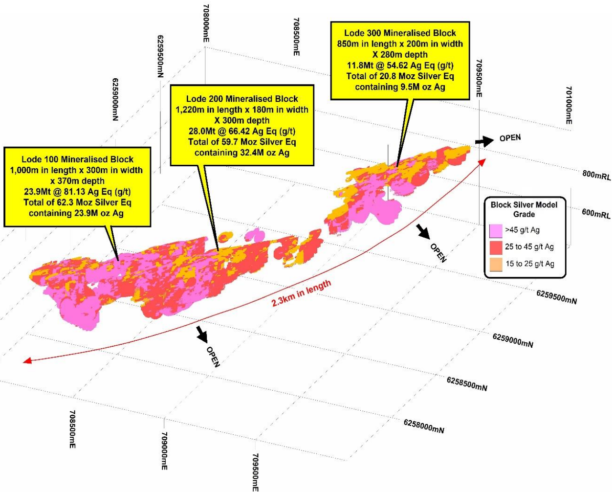
Figure 7 – Oblique 3D Image looking NW of Kempfield outlining the Dimensions & Grade of Mineralised Block Model
