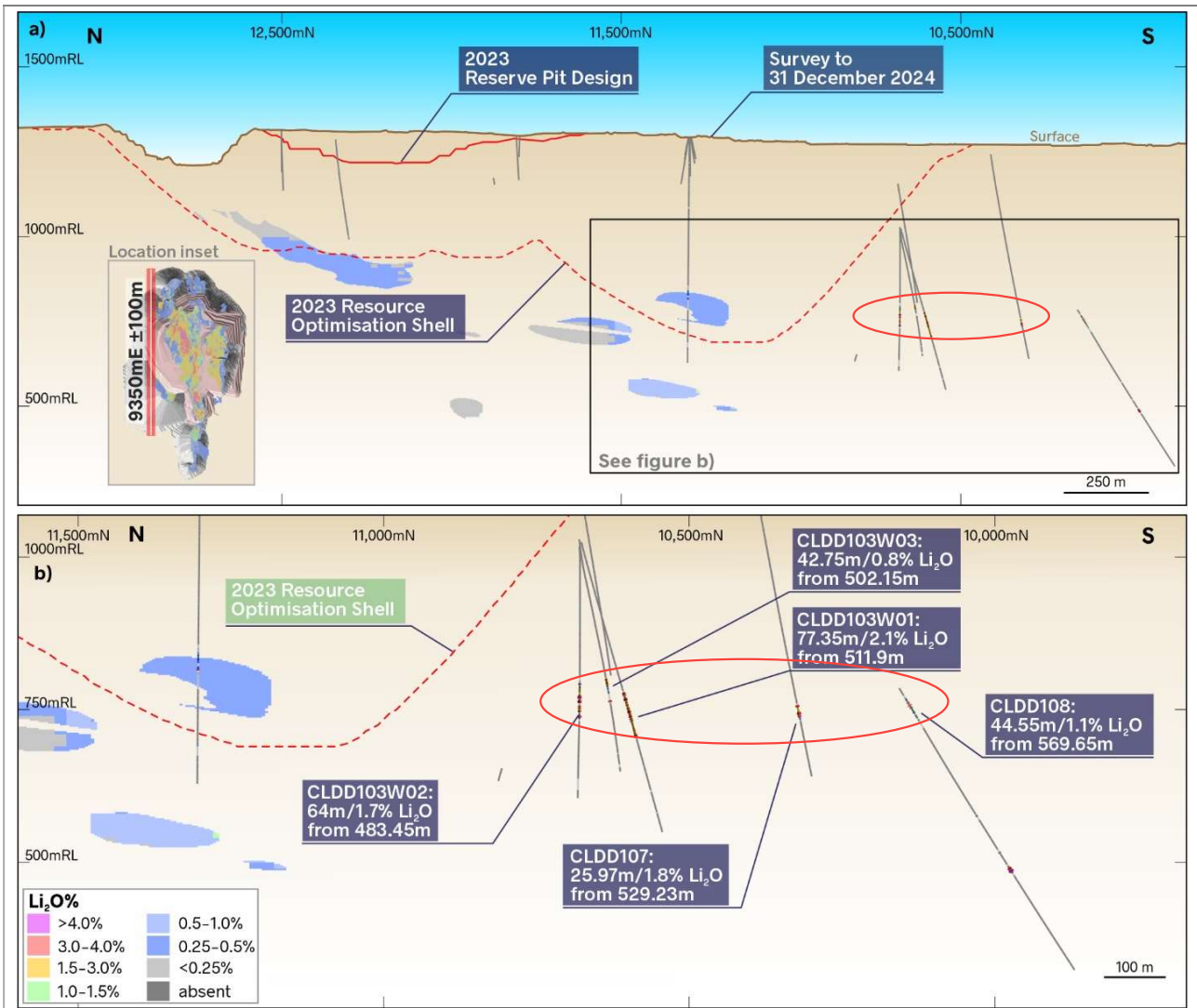
Figure 8: Central Lode long section 9,350mE ± 100m with example CY24 drilling results
