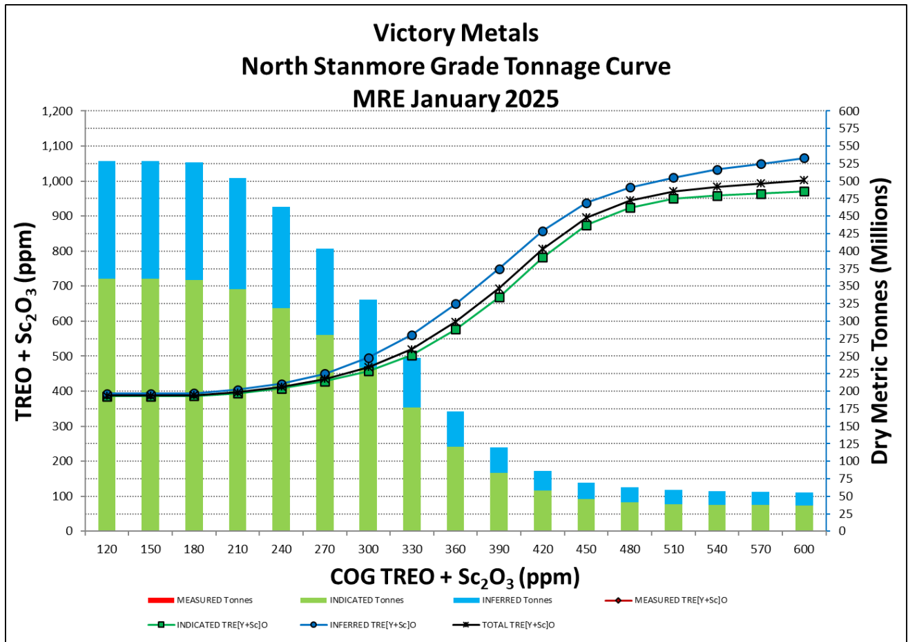
Figure 3: Grade tonnage curve for the North Stanmore TREO + \text{Sc}_2\text{O}_3 MRE (Indicated and Inferred)
