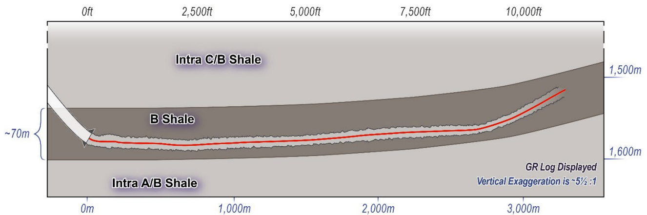
Carpentaria-5H Horizontal Section Schematic
