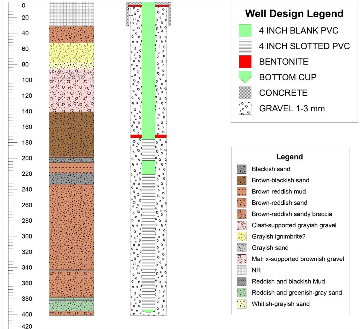
Figure 4. Log of sediments and well design with 4inch PVC lining. Porous sediments and volcanics (a source of lithium) start at 60m and brown reddish sandy Breccia is open at depth.
