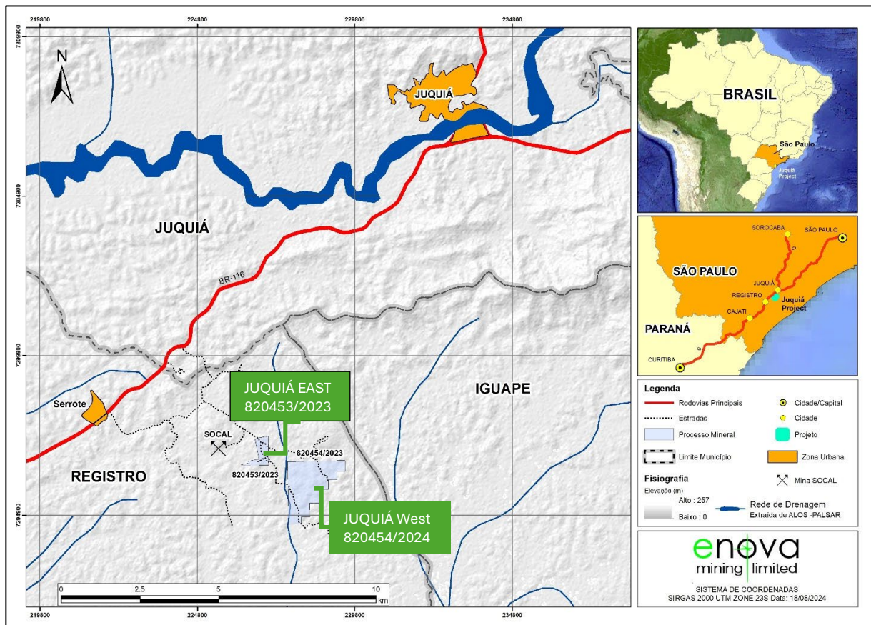
Figure 12: The Juquiá Alkaline Complex project tenements (100% ENV) Sao Paulo, Brazil
