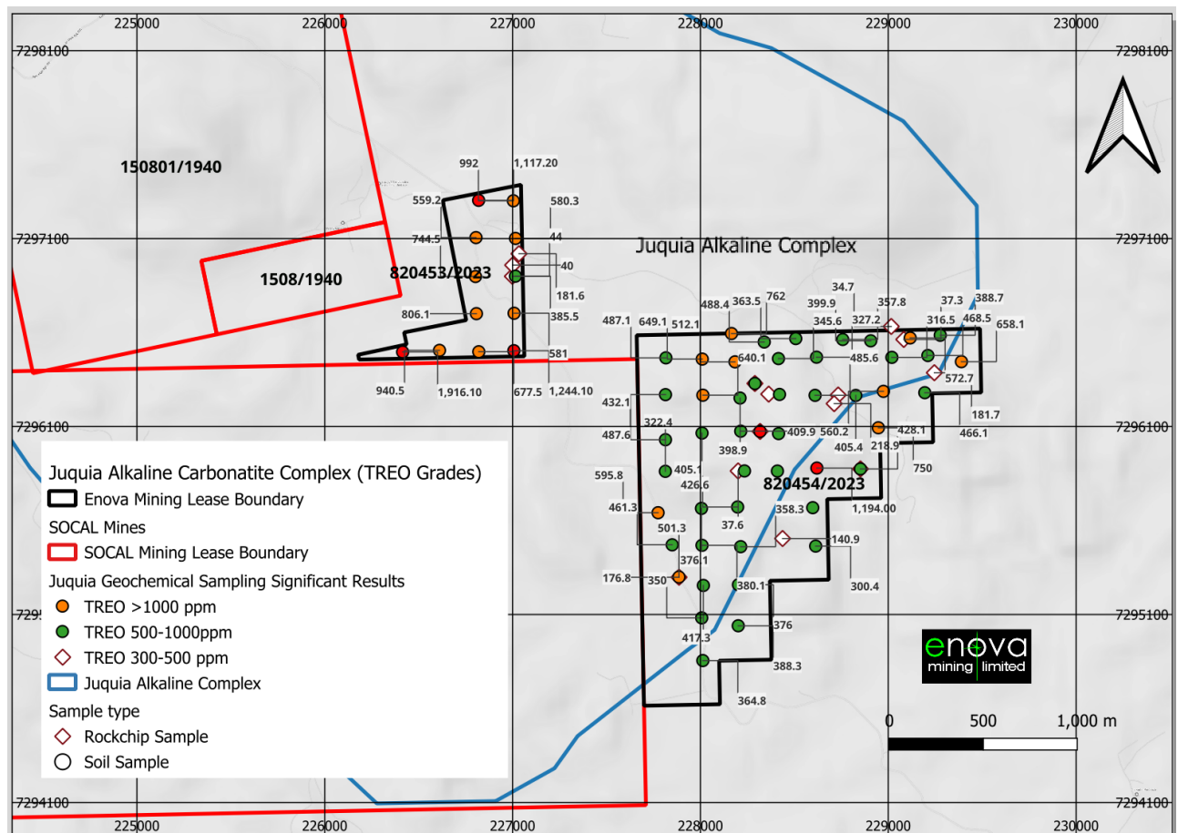
Figure 10: Surface Geochemical sample points and TREO anomalous assay results at Juquiá Alkaline Complex
