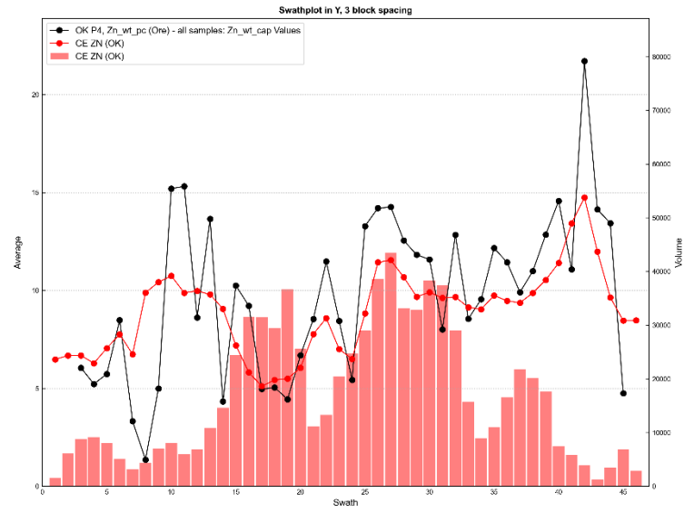
Figure 4. Swath Plots in Y for Zn grades. The black dotted line shows the average Zn grade of the samples for each slice, the red dotted line shows the average Zn grade of the estimated blocks for each slice, and the histogram (in red) indicates the volume of blocks in each slice.
