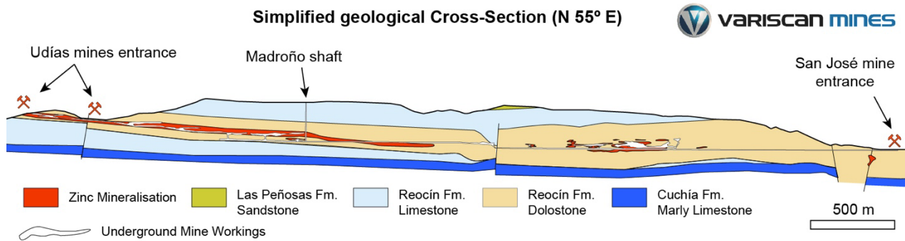
Figure 10. Simplified geological cross-section showing connectivity and continuity between San Jose Mine and Udias Mine (refer ASX Announcement 10 September 2024)
