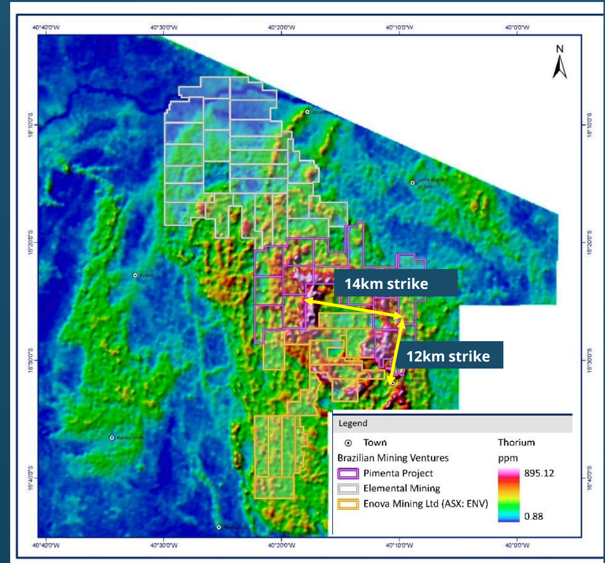
Thorium radiometric imaging showing circular intrusive signature over Pimento tenements
