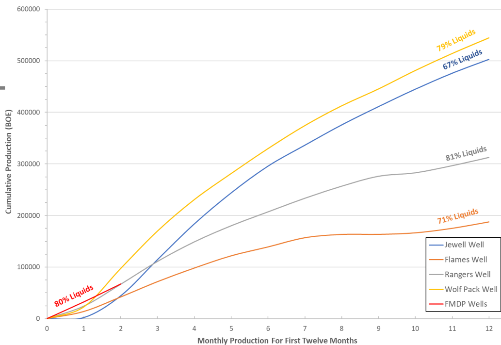
Figure 1. Cumulative production for SWISH operated wells normalised to a notional 10,000-foot lateral.
