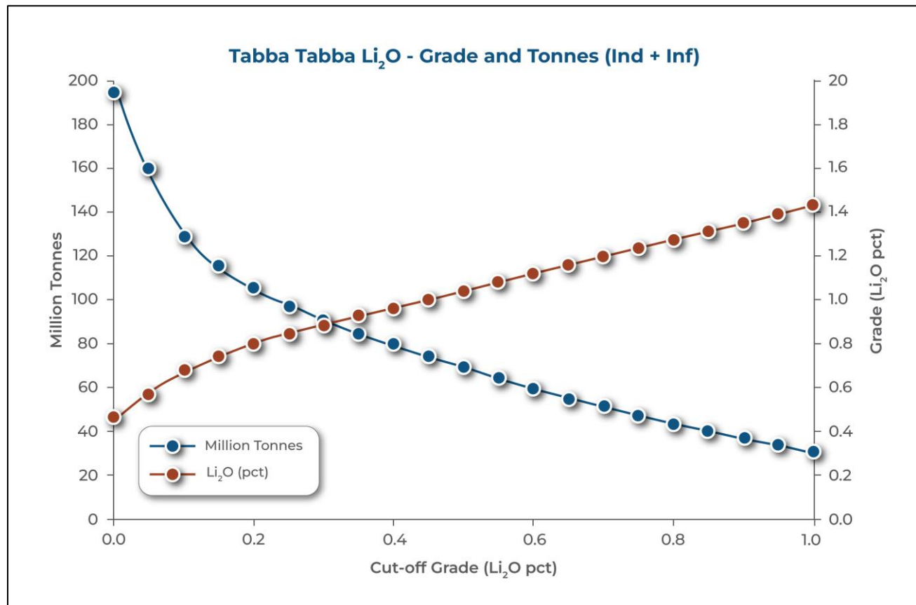
Figure 3 – Tabba Tabba Lithium Project Grade Tonnage Curve
