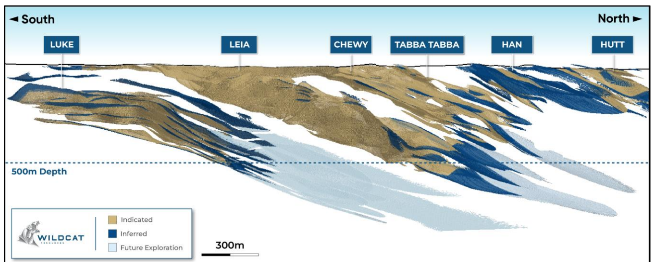
Figure 1 – Isometric of Indicated and Inferred Mineral Resource classifications at Tabba Tabba Lithium project with plunge extents identified as targets for future exploration drilling.
