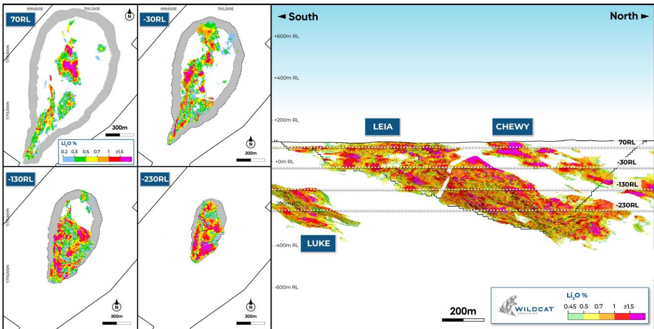
Figure 7 – 100m thick Flitch Plans (>0.2% Li 2 O) through a west looking view of a conceptual pit at Leia of the Tabba Tabba lithium block model (>0.45% Li 2 O).
