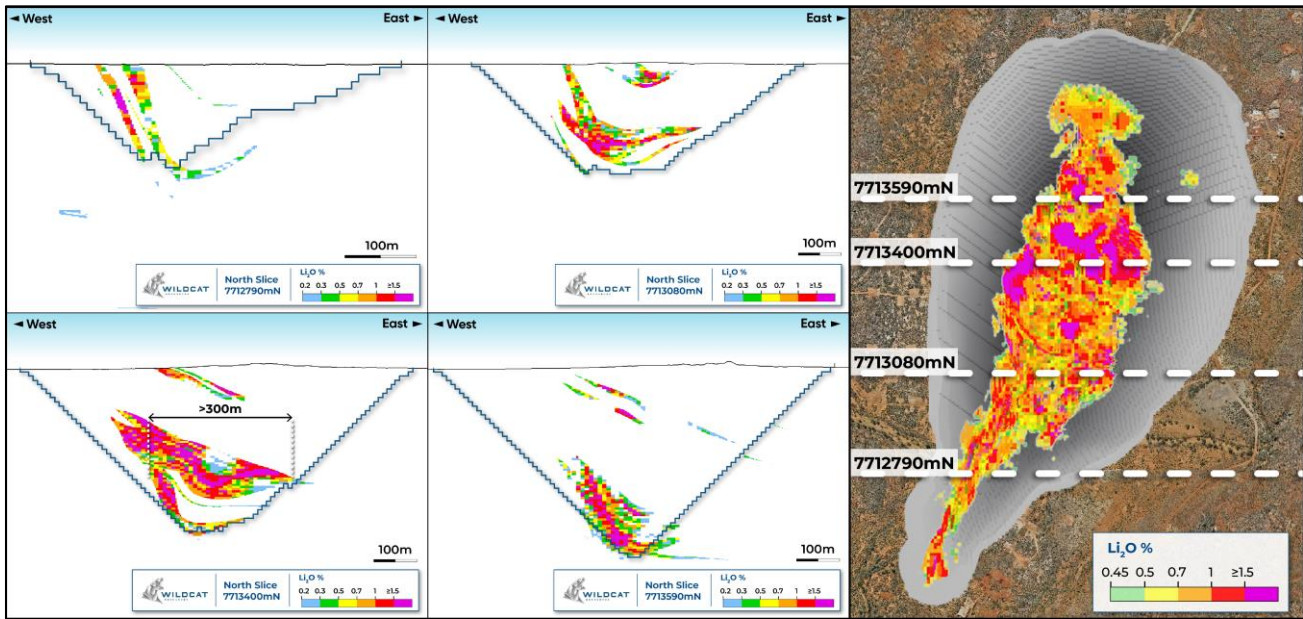
Figure 6 – Cross Sections (>0.2% Li 2 O) through a plan view of a conceptual pit at Leia of the Tabba Tabba lithium block model (>0.45% Li 2 O).
