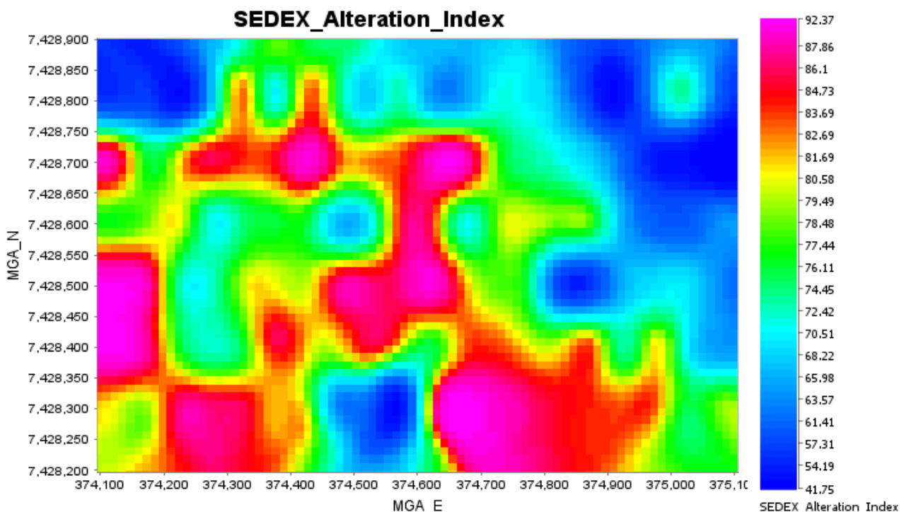
Figure 6. Gridded “SEDEX Alteration Index”.
