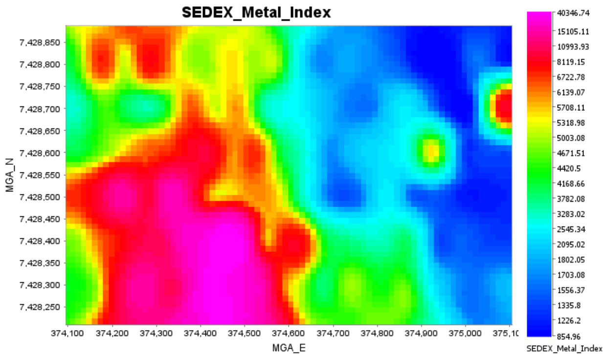
Figure 5. Gridded “SEDEX Metal Index”.
