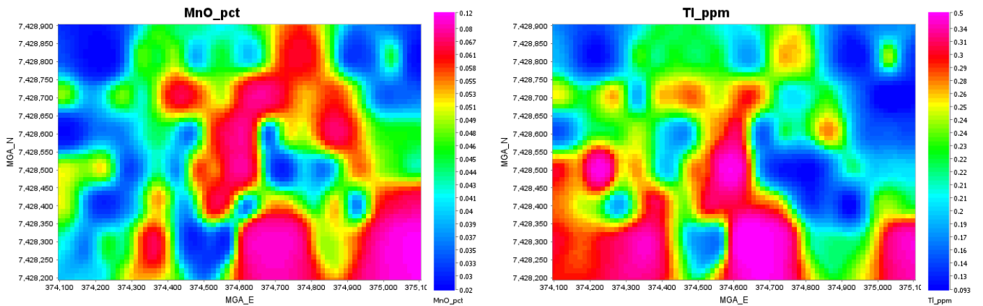
Figure 3. Gridded soil results for MnO and TI.
