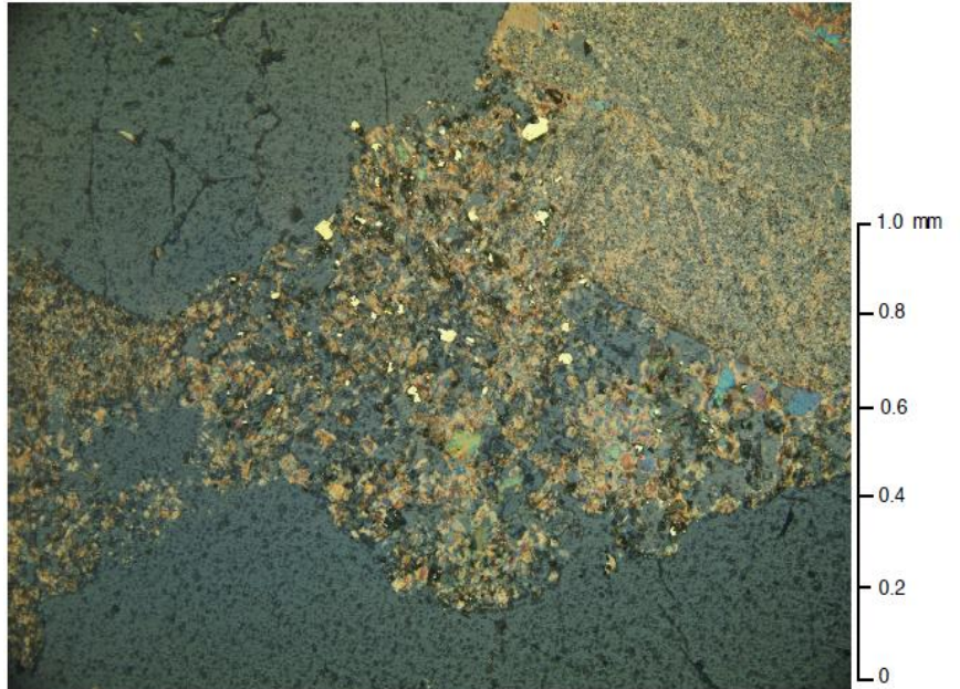
FIG. 4: SAMPLE SOMDD002_69.5m (Combined transmitted and reflected light, crossed polarisers, Image P6068583) This view illustrates a cloud of tiny bright yellow native gold grains 2-30 µm in size which are disseminated through fine-grained sericite (small dull colourful flakes) after a plagioclase grain. Larger quartz grains are clear and unaltered (dull grey; top left, bottom).
