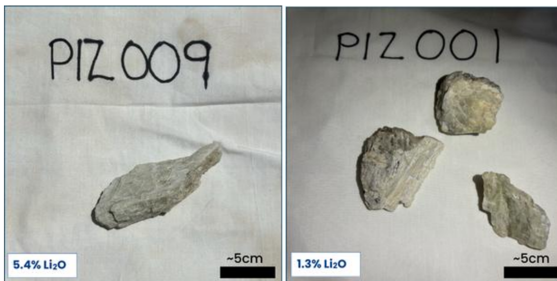
Figure 5: Spodumene sample & relating assay result 9 .
