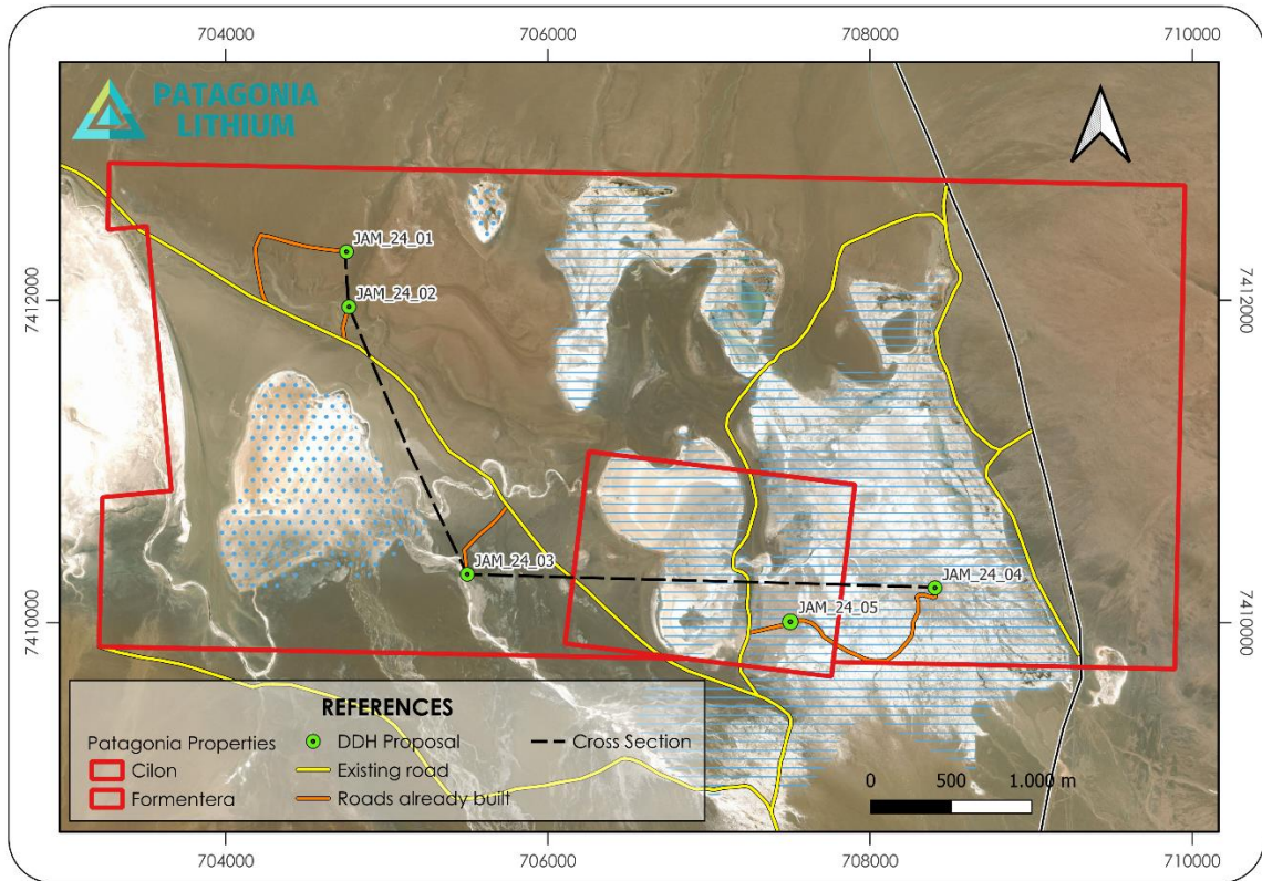
Figure 4. The location of JAM24-05 drill well is shown above on the Cilon concession of 200Has.
