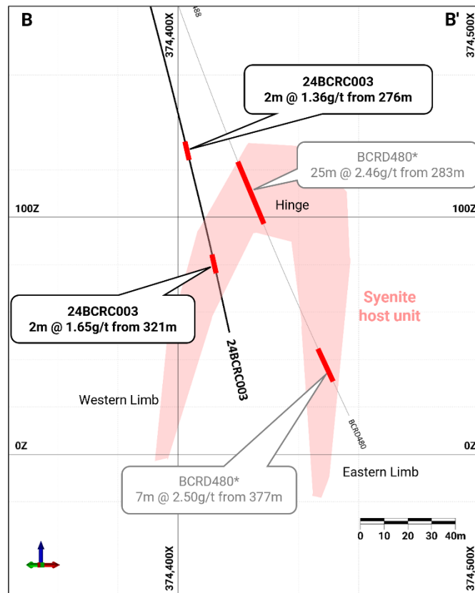
Figure 3 - 24BCRC003 drill section (* denotes historic drillhole)
