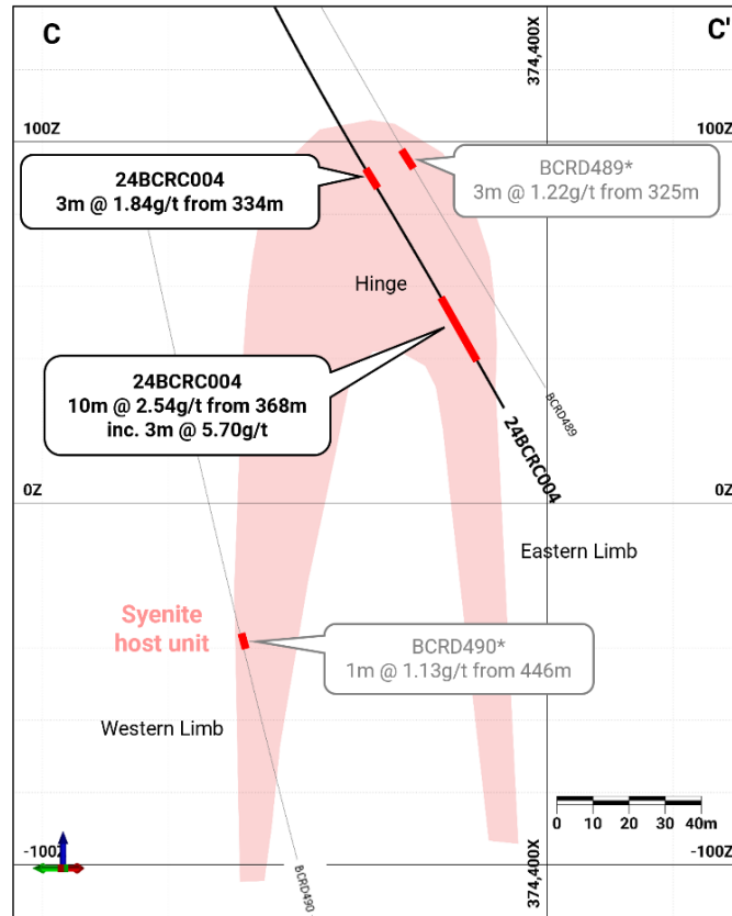
Figure 4 - 24BCRC004 drill section (*denotes historic drillhole)
