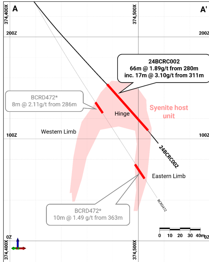
Figure 2 - 24BCRC002 drill section (*denotes historic drillhole)
