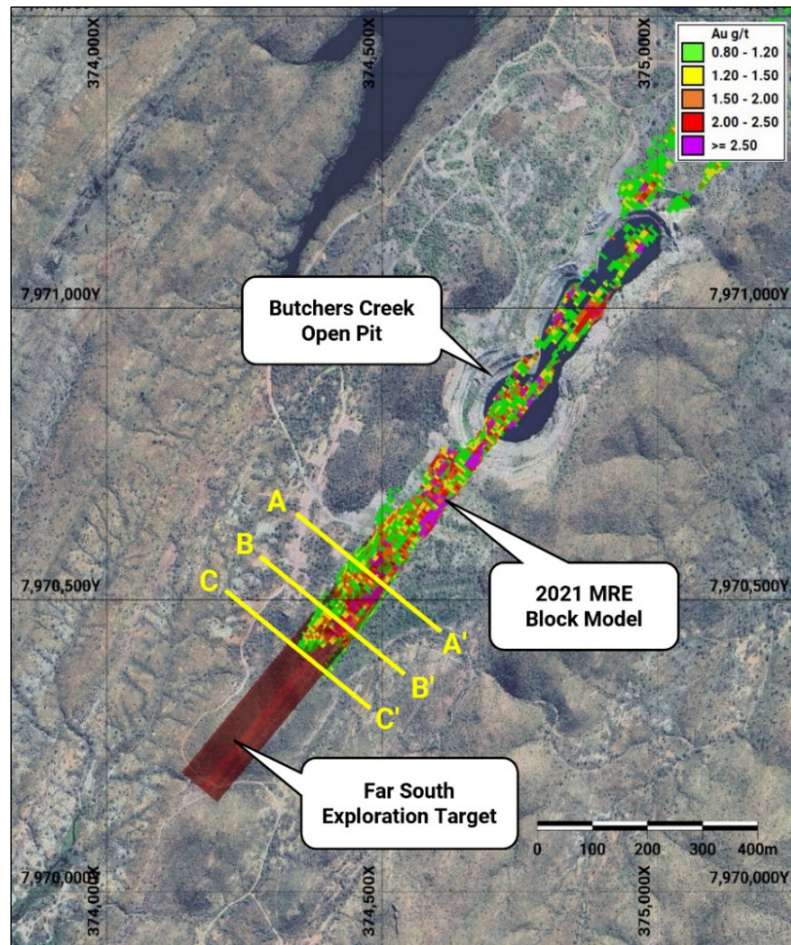
Figure 1 - Plan view of Butchers Creek with related drill section lines
