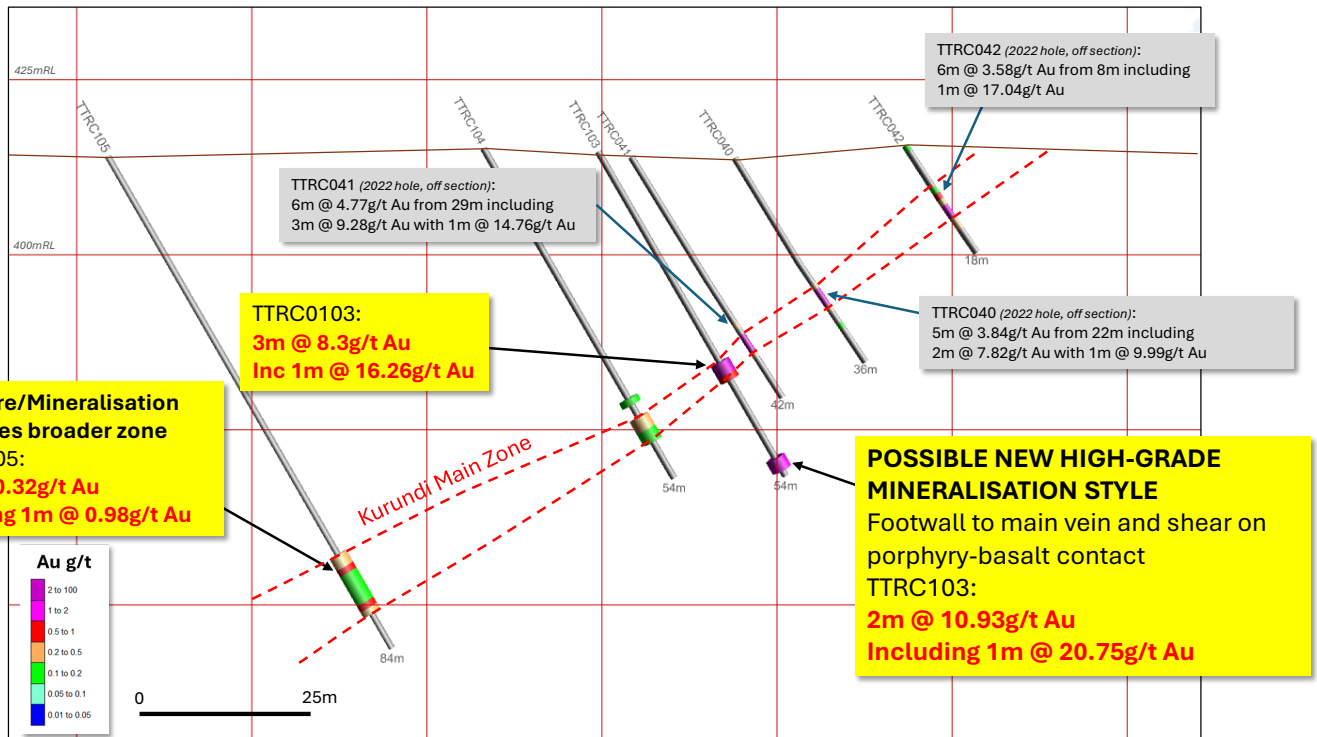
Figure 3: Cross Section (oblique section, location shown in Figure 4) showing holes near to the new high grade mineralisation footwall to the Kurundi Central main zone, TTRC040-42 are 2022 holes off section.
