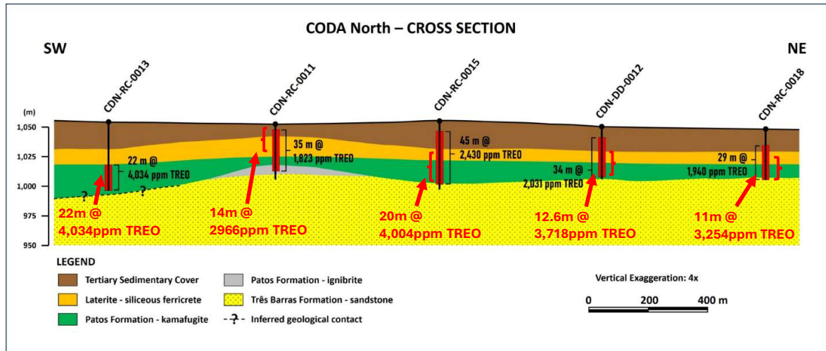
Figure 5: Schematic cross section (only significant values such as maximum intercepts and high grades of the current announcement are shown)
