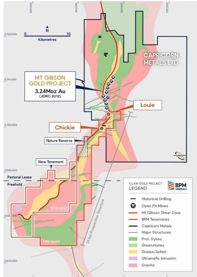
Fig. 6 - Claw Project - Regional Geology
